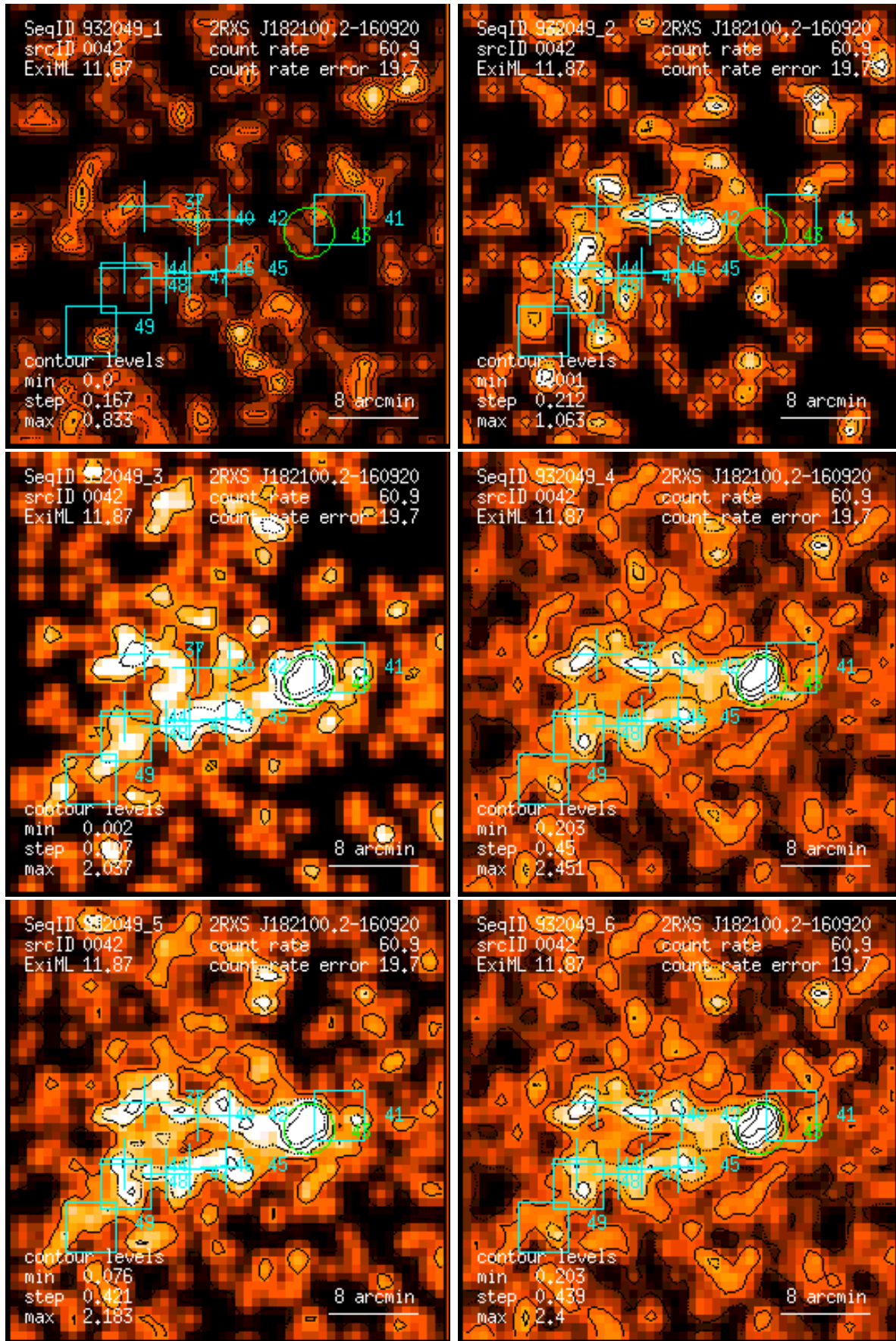
Figure 42: RASS 932049: detection 0042: band rate images, Gaussian filter: (1) PSPC channels 11 – 41, (2) 52 – 90, (3) 91 – 201, (4) 11 – 235, (5) 52 – 201, (6) 11 – 201. Broad band rates in counts/ks. Band rate contour levels in counts/ks/arcmin 2 .
