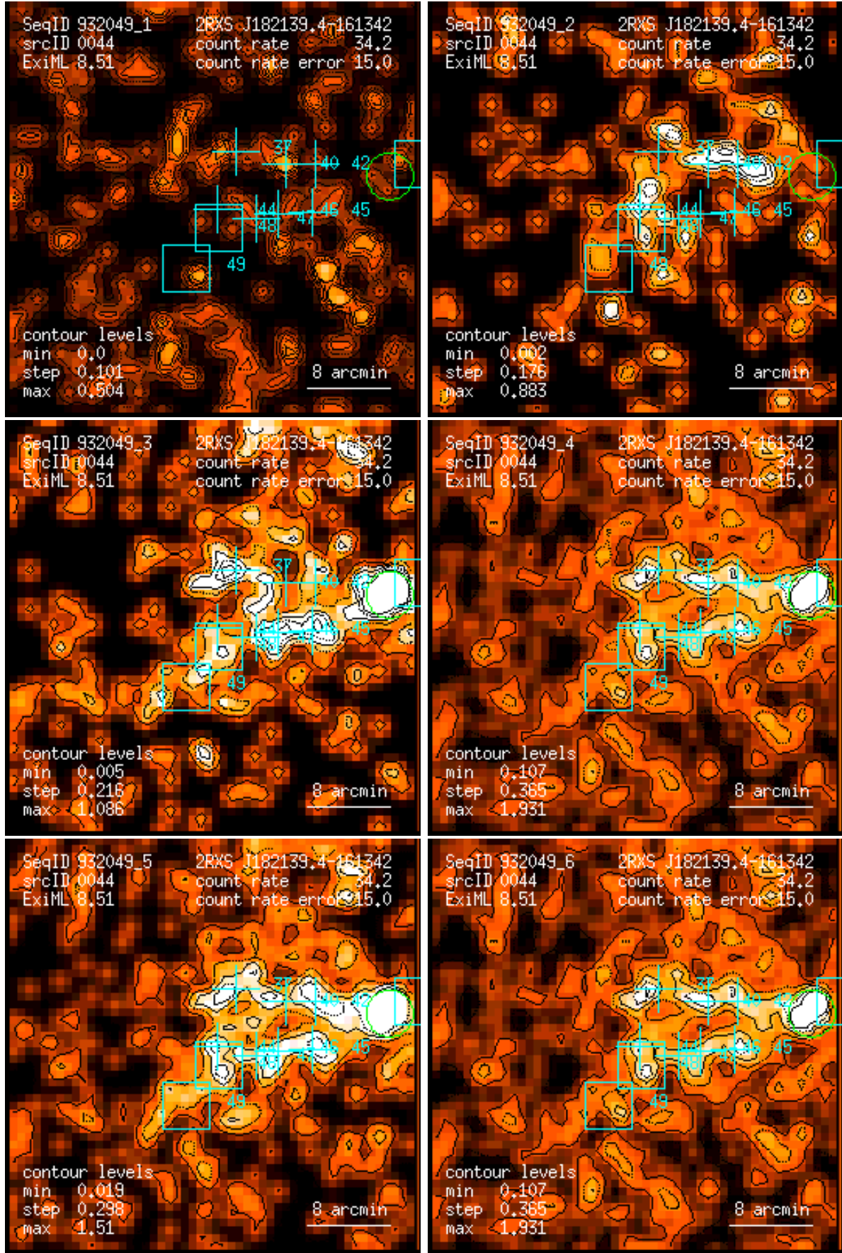
Figure 44: RASS 932049: detection 0044: band rate images, Gaussian filter: (1) PSPC channels 11 – 41, (2) 52 – 90, (3) 91 – 201, (4) 11 – 235, (5) 52 – 201, (6) 11 – 201. Broad band rates in counts/ks. Band rate contour levels in counts/ks/arcmin 2 .
