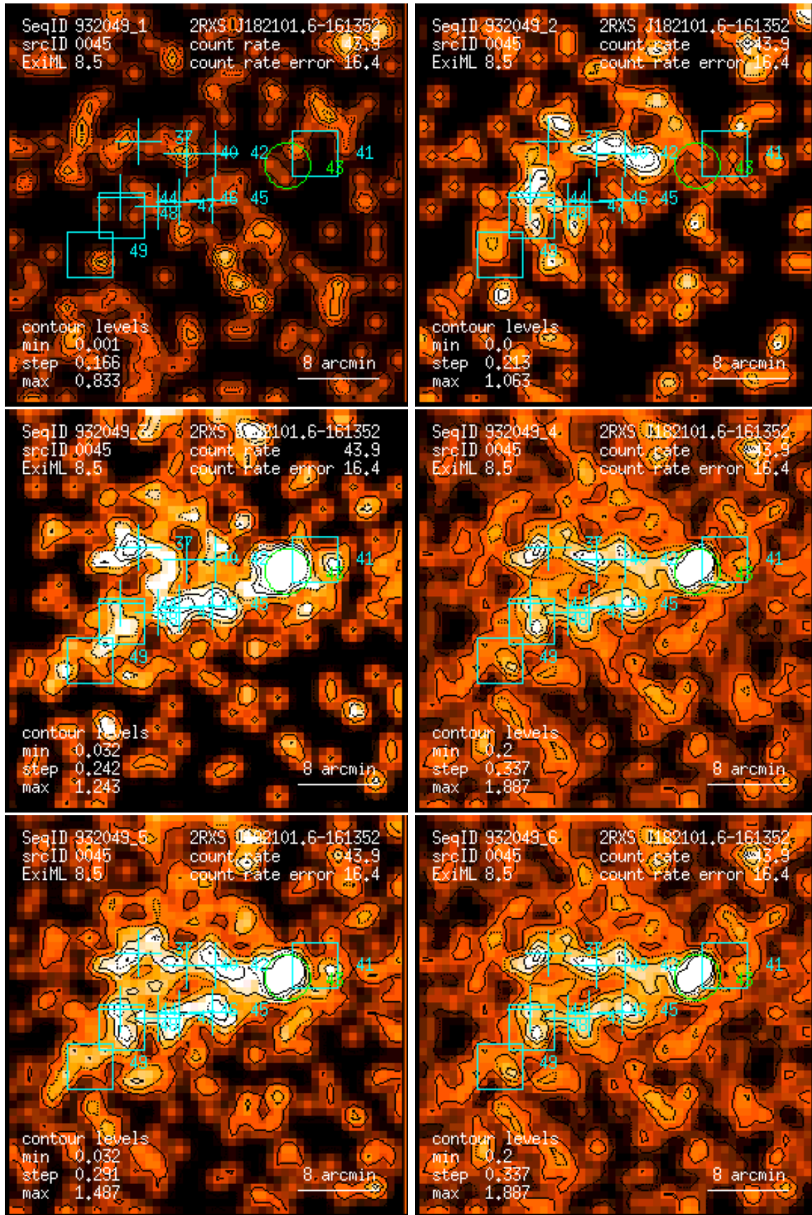
Figure 45: RASS 932049: detection 0045: band rate images, Gaussian filter: (1) PSPC channels 11 – 41, (2) 52 – 90, (3) 91 – 201, (4) 11 – 235, (5) 52 – 201, (6) 11 – 201. Broad band rates in counts/ks. Band rate contour levels in counts/ks/arcmin 2 .
