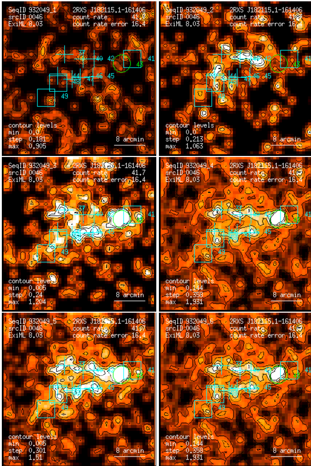
Figure 46: RASS 932049: detection 0046: band rate images, Gaussian filter: (1) PSPC channels 11 – 41, (2) 52 – 90, (3) 91 – 201, (4) 11 – 235, (5) 52 – 201, (6) 11 – 201. Broad band rates in counts/ks. Band rate contour levels in counts/ks/arcmin 2 .
