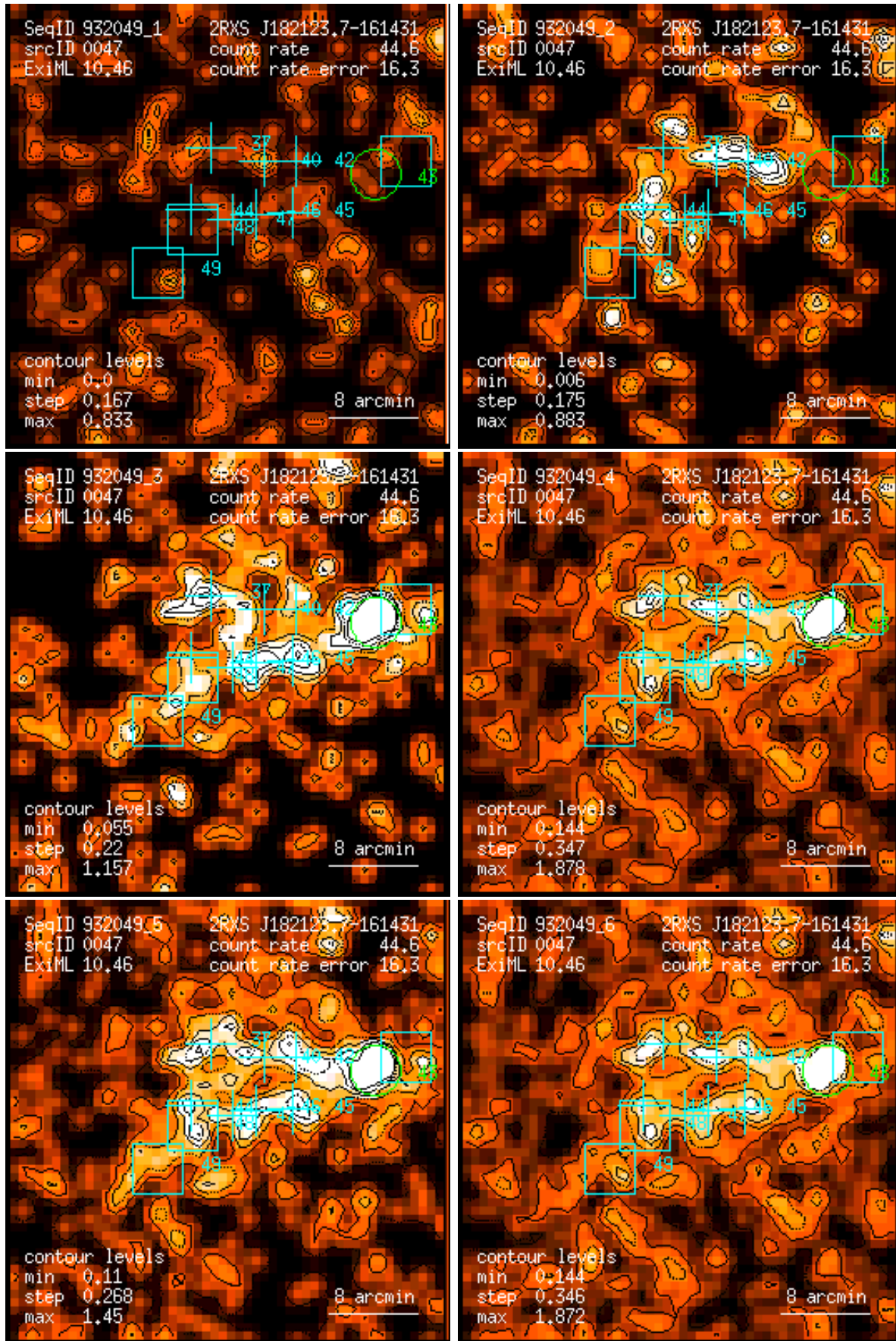
Figure 47: RASS 932049: detection 0047: band rate images, Gaussian filter: (1) PSPC channels 11 – 41, (2) 52 – 90, (3) 91 – 201, (4) 11 – 235, (5) 52 – 201, (6) 11 – 201. Broad band rates in counts/ks. Band rate contour levels in counts/ks/arcmin 2 .
