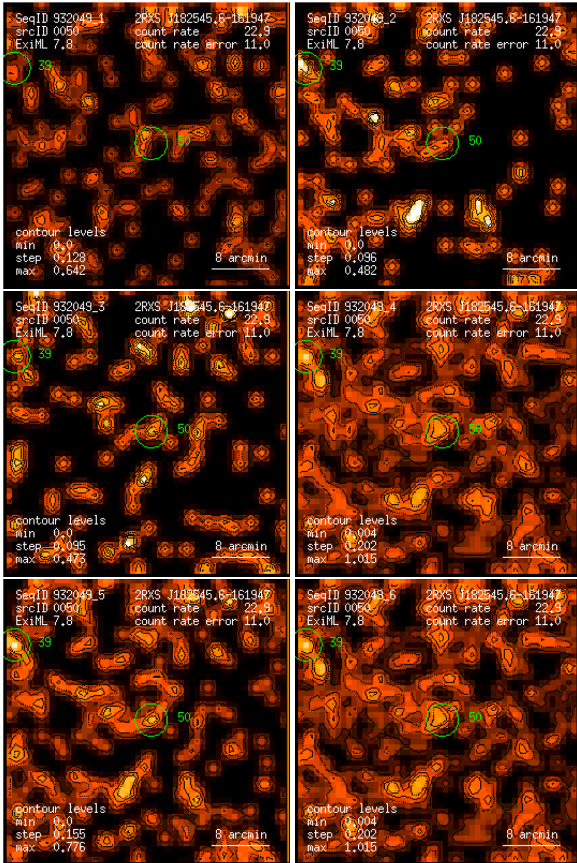
Figure 50: RASS 932049: detection 0050: band rate images, Gaussian filter: (1) PSPC channels 11 – 41, (2) 52 – 90, (3) 91 – 201, (4) 11 – 235, (5) 52 – 201, (6) 11 – 201. Broad band rates in counts/ks. Band rate contour levels in counts/ks/arcmin 2 .
