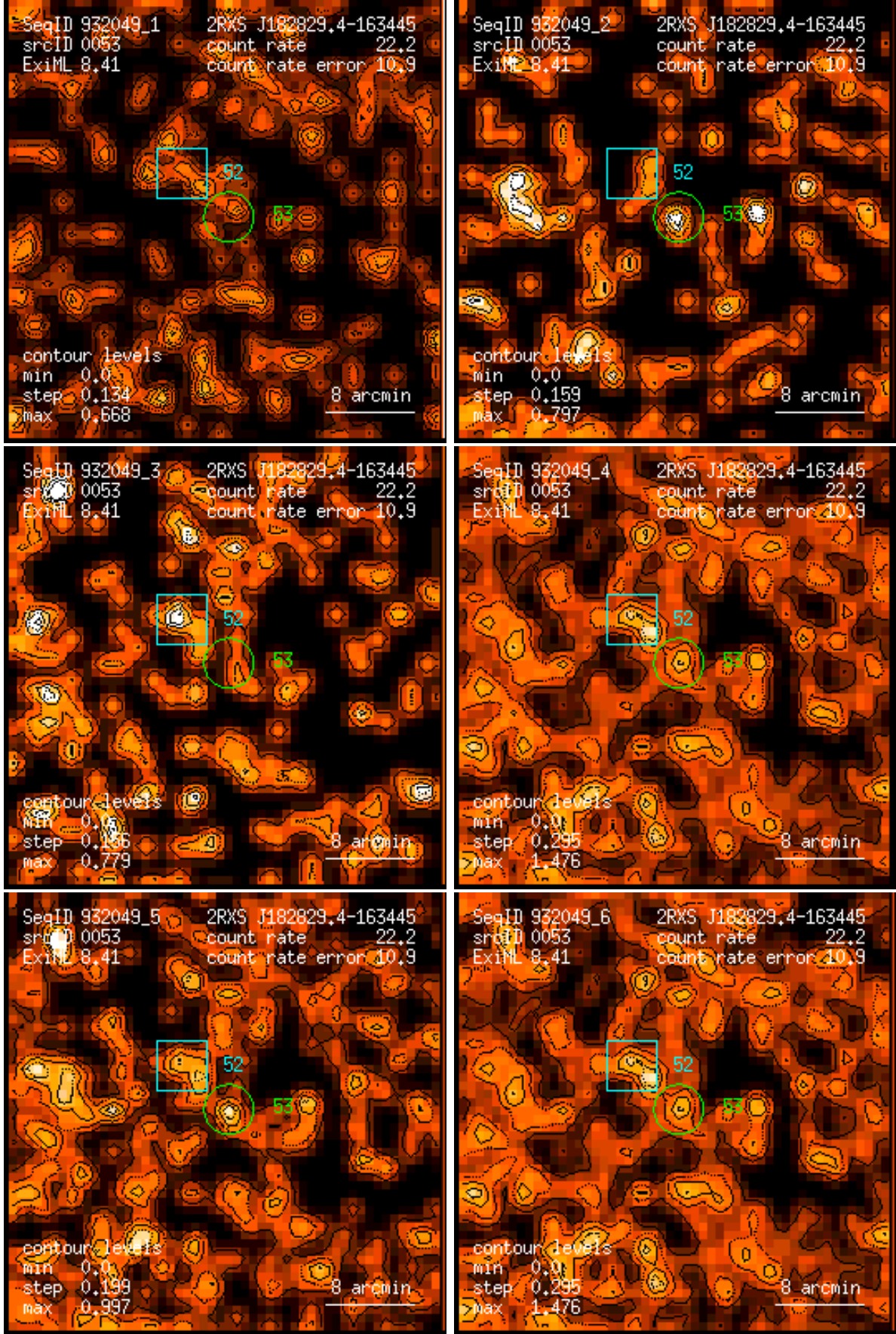
Figure 53: RASS 932049: detection 0053: band rate images, Gaussian filter: (1) PSPC channels 11 – 41, (2) 52 – 90, (3) 91 – 201, (4) 11 – 235, (5) 52 – 201, (6) 11 – 201. Broad band rates in counts/ks. Band rate contour levels in counts/ks/arcmin 2 .
