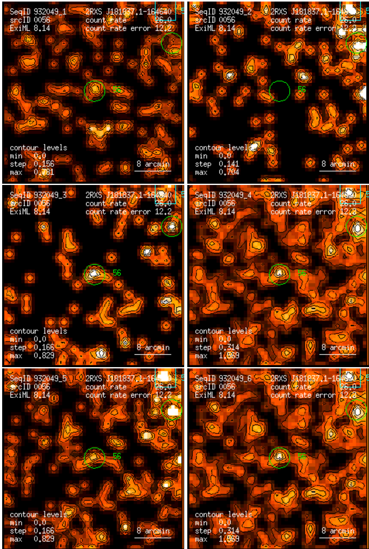
Figure 56: RASS 932049: detection 0056: band rate images, Gaussian filter: (1) PSPC channels 11 – 41, (2) 52 – 90, (3) 91 – 201, (4) 11 – 235, (5) 52 – 201, (6) 11 – 201. Broad band rates in counts/ks. Band rate contour levels in counts/ks/arcmin 2 .
