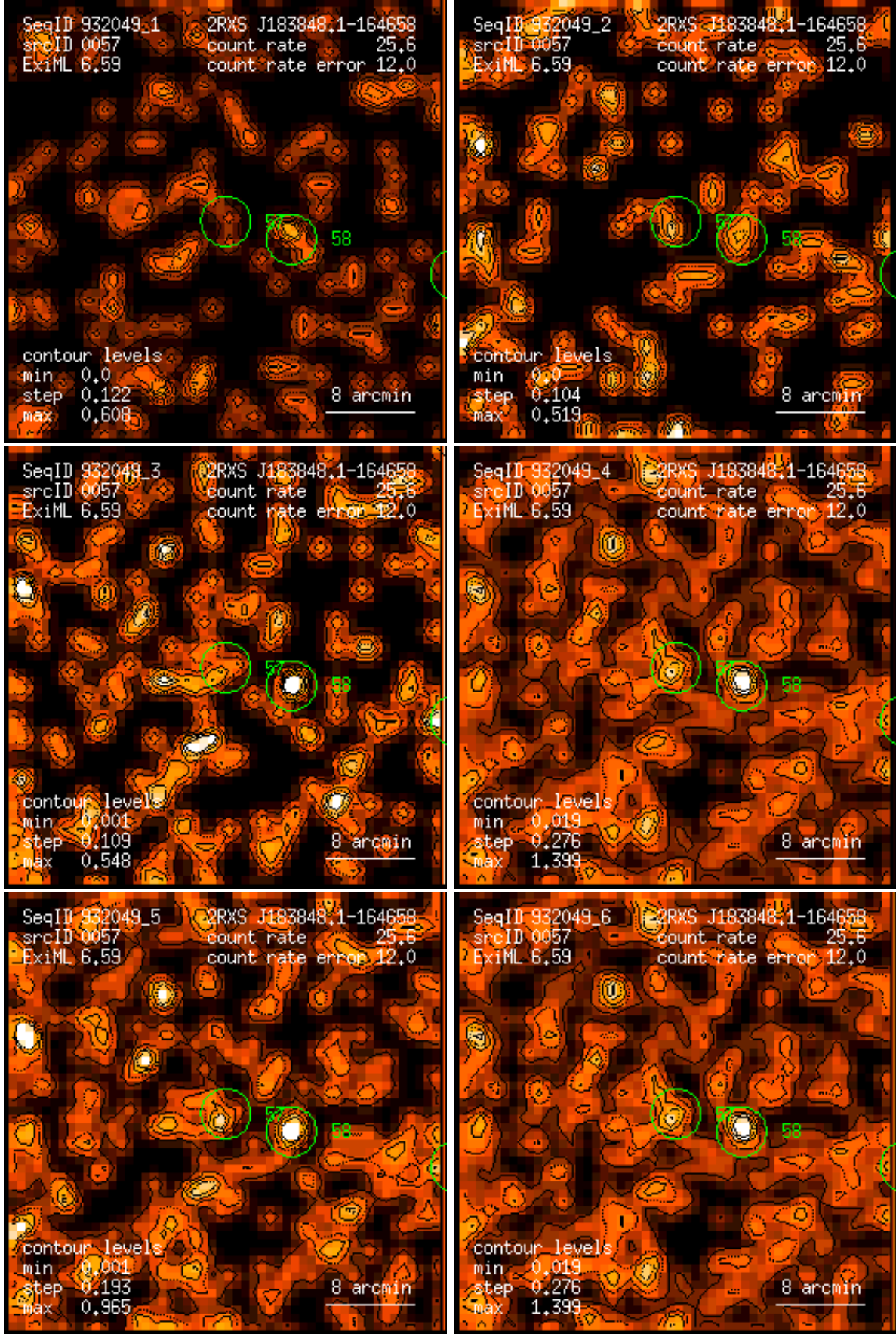
Figure 57: RASS 932049: detection 0057: band rate images, Gaussian filter: (1) PSPC channels 11 – 41, (2) 52 – 90, (3) 91 – 201, (4) 11 – 235, (5) 52 – 201, (6) 11 – 201. Broad band rates in counts/ks. Band rate contour levels in counts/ks/arcmin 2 .
