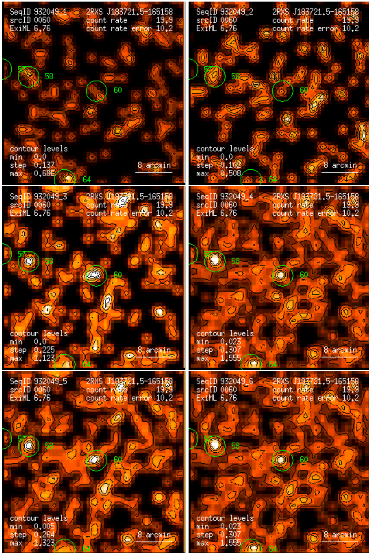
Figure 60: RASS 932049: detection 0060: band rate images, Gaussian filter: (1) PSPC channels 11 – 41, (2) 52 – 90, (3) 91 – 201, (4) 11 – 235, (5) 52 – 201, (6) 11 – 201. Broad band rates in counts/ks. Band rate contour levels in counts/ks/arcmin 2 .
