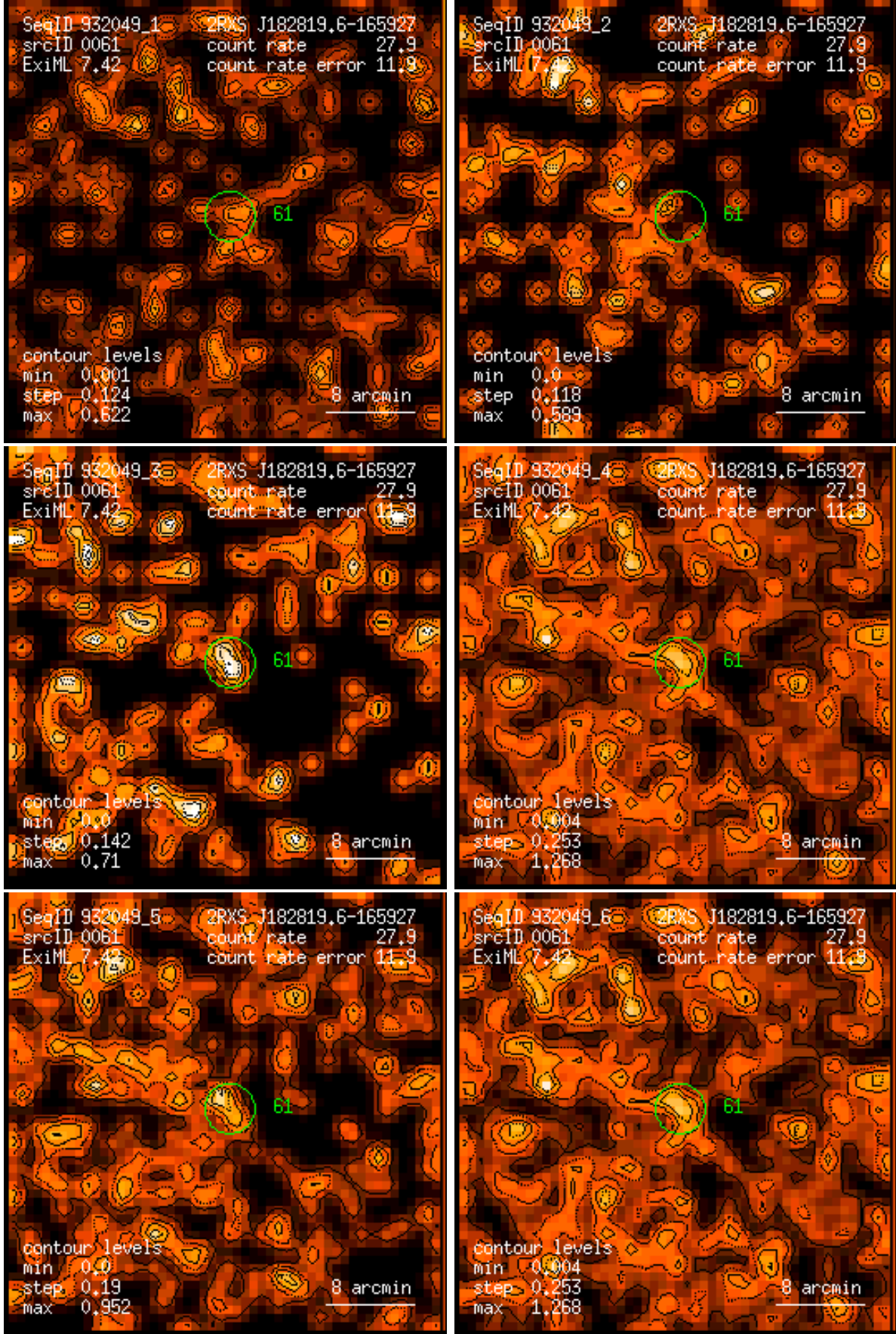
Figure 61: RASS 932049: detection 0061: band rate images, Gaussian filter: (1) PSPC channels 11 – 41, (2) 52 – 90, (3) 91 – 201, (4) 11 – 235, (5) 52 – 201, (6) 11 – 201. Broad band rates in counts/ks. Band rate contour levels in counts/ks/arcmin 2 .
