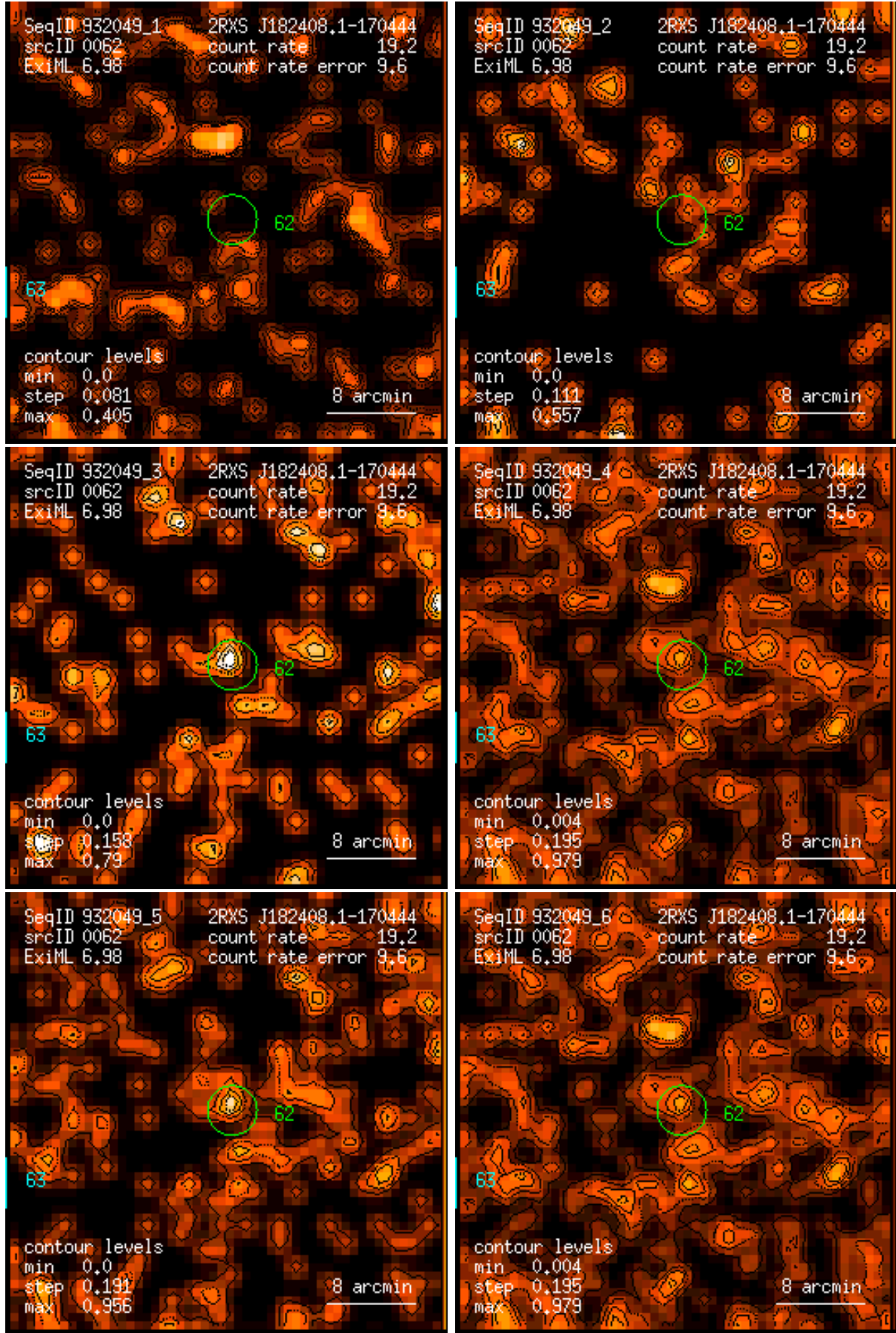
Figure 62: RASS 932049: detection 0062: band rate images, Gaussian filter: (1) PSPC channels 11 – 41, (2) 52 – 90, (3) 91 – 201, (4) 11 – 235, (5) 52 – 201, (6) 11 – 201. Broad band rates in counts/ks. Band rate contour levels in counts/ks/arcmin 2 .
