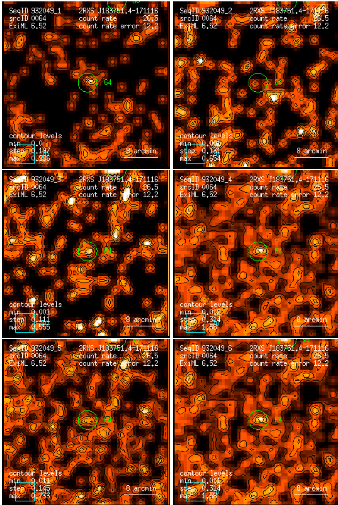
Figure 64: RASS 932049: detection 0064: band rate images, Gaussian filter: (1) PSPC channels 11 – 41, (2) 52 – 90, (3) 91 – 201, (4) 11 – 235, (5) 52 – 201, (6) 11 – 201. Broad band rates in counts/ks. Band rate contour levels in counts/ks/arcmin 2 .
