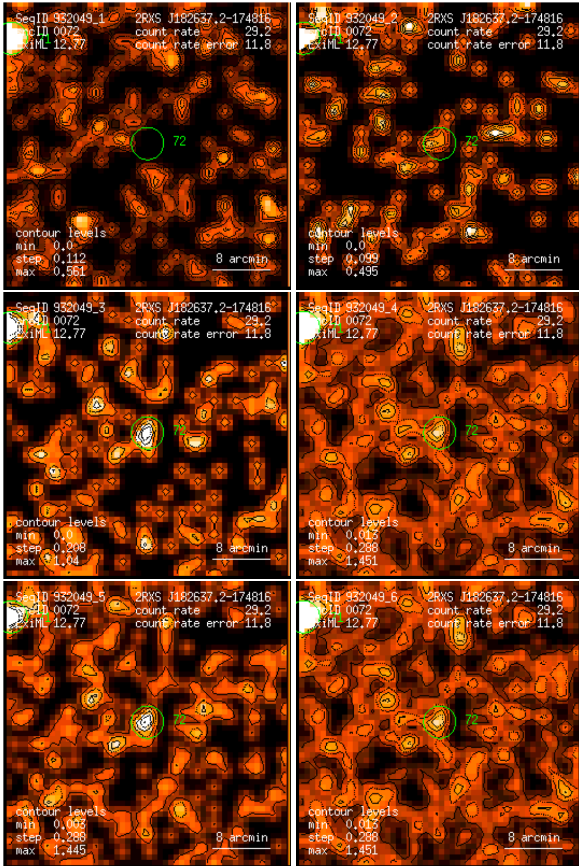
Figure 72: RASS 932049: detection 0072: band rate images, Gaussian filter: (1) PSPC channels 11 – 41, (2) 52 – 90, (3) 91 – 201, (4) 11 – 235, (5) 52 – 201, (6) 11 – 201. Broad band rates in counts/ks. Band rate contour levels in counts/ks/arcmin 2 .
