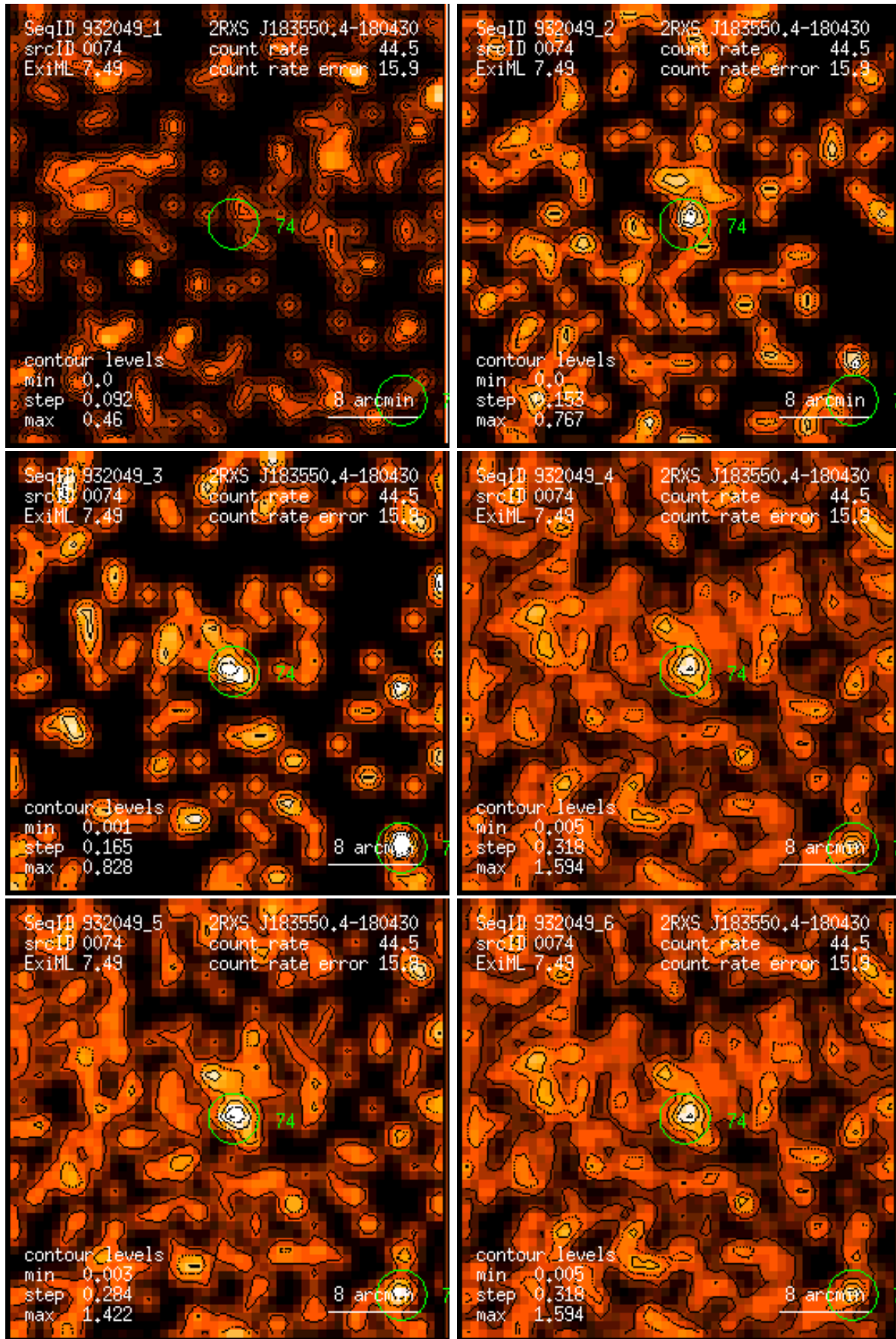
Figure 74: RASS 932049: detection 0074: band rate images, Gaussian filter: (1) PSPC channels 11 – 41, (2) 52 – 90, (3) 91 – 201, (4) 11 – 235, (5) 52 – 201, (6) 11 – 201. Broad band rates in counts/ks. Band rate contour levels in counts/ks/arcmin 2 .
