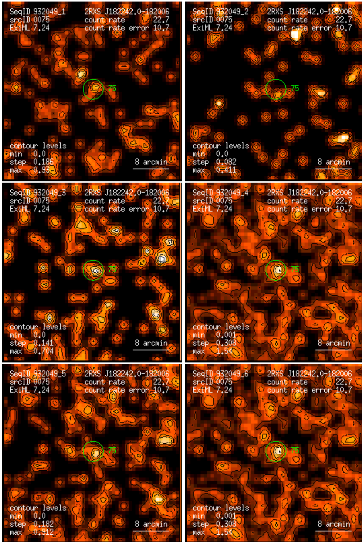
Figure 75: RASS 932049: detection 0075: band rate images, Gaussian filter: (1) PSPC channels 11 – 41, (2) 52 – 90, (3) 91 – 201, (4) 11 – 235, (5) 52 – 201, (6) 11 – 201. Broad band rates in counts/ks. Band rate contour levels in counts/ks/arcmin 2 .
