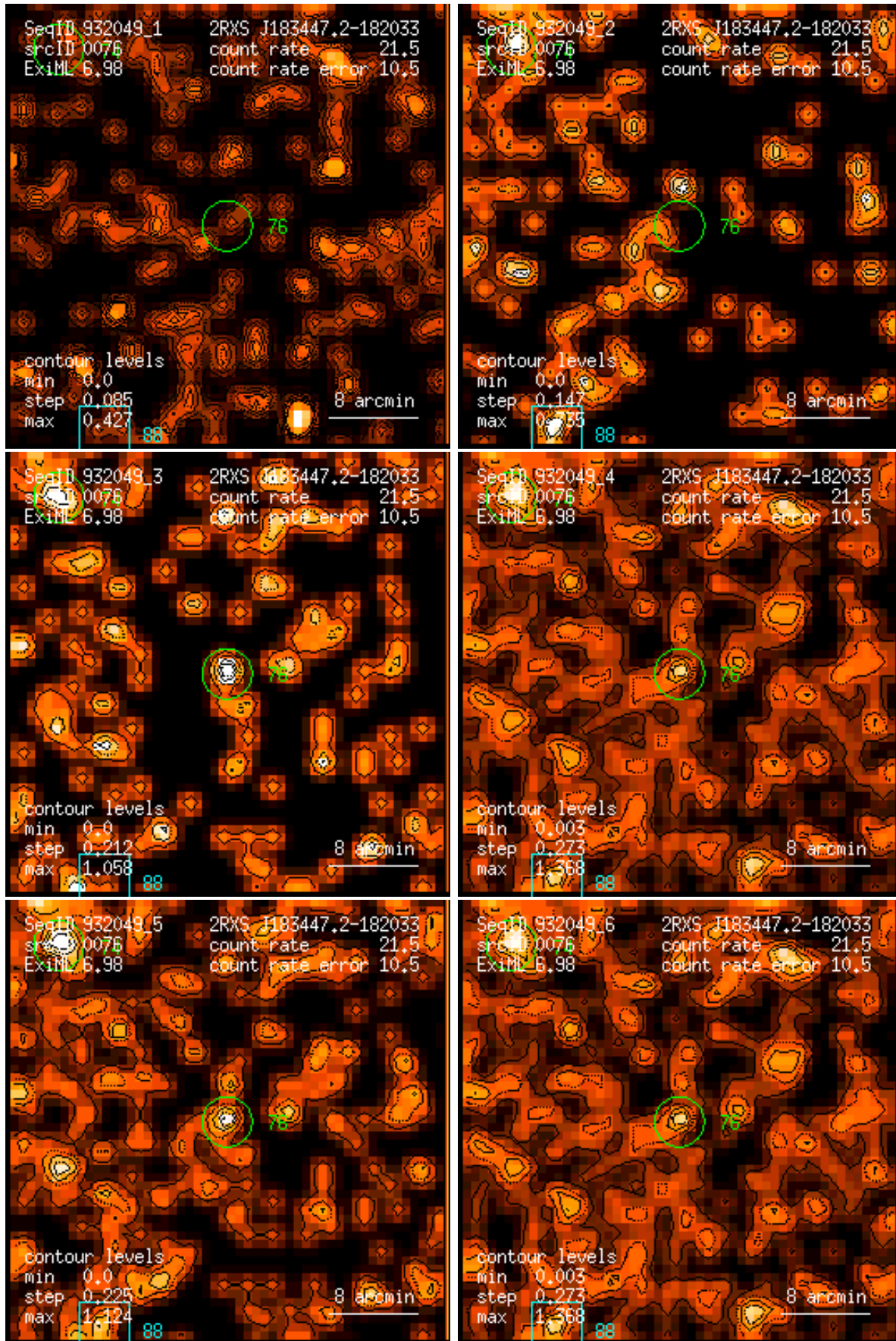
Figure 76: RASS 932049: detection 0076: band rate images, Gaussian filter: (1) PSPC channels 11 – 41, (2) 52 – 90, (3) 91 – 201, (4) 11 – 235, (5) 52 – 201, (6) 11 – 201. Broad band rates in counts/ks. Band rate contour levels in counts/ks/arcmin 2 .
