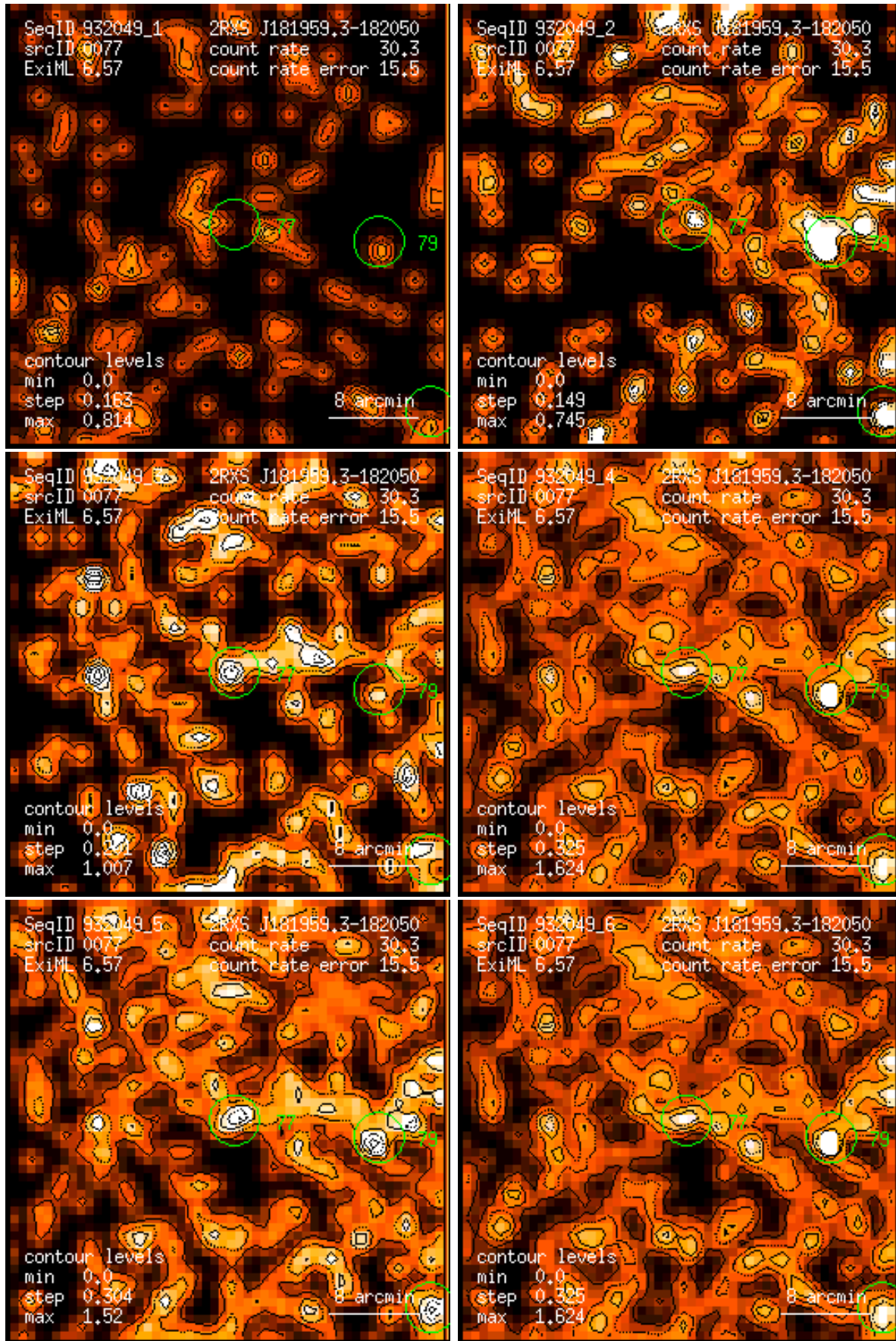
Figure 77: RASS 932049: detection 0077: band rate images, Gaussian filter: (1) PSPC channels 11 – 41, (2) 52 – 90, (3) 91 – 201, (4) 11 – 235, (5) 52 – 201, (6) 11 – 201. Broad band rates in counts/ks. Band rate contour levels in counts/ks/arcmin 2 .
