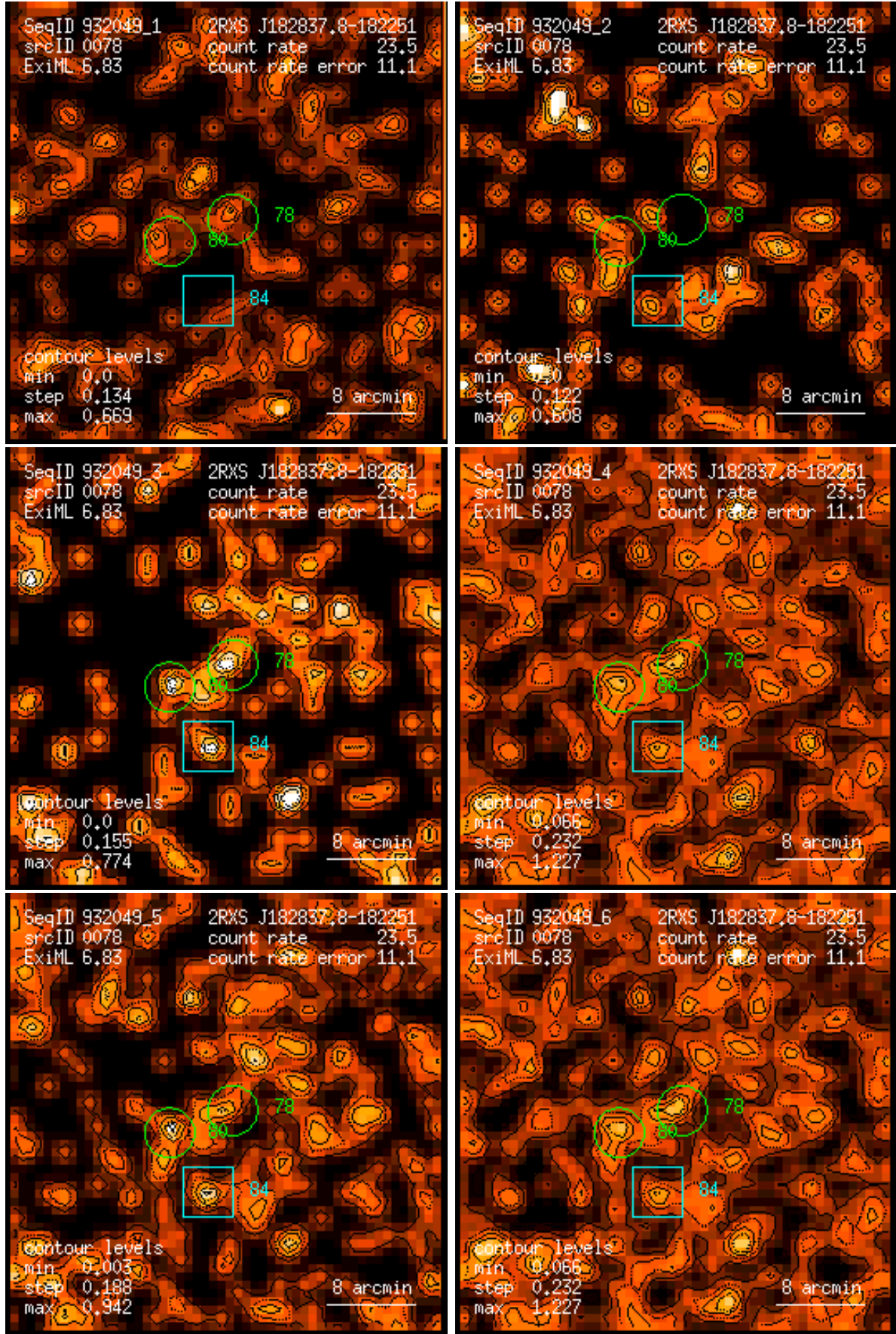
Figure 78: RASS 932049: detection 0078: band rate images, Gaussian filter: (1) PSPC channels 11 – 41, (2) 52 – 90, (3) 91 – 201, (4) 11 – 235, (5) 52 – 201, (6) 11 – 201. Broad band rates in counts/ks. Band rate contour levels in counts/ks/arcmin 2 .
