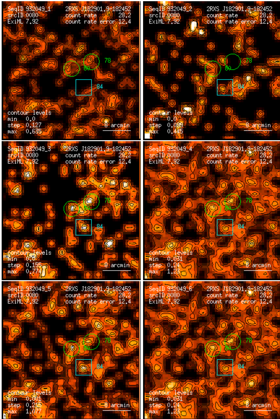
Figure 80: RASS 932049: detection 0080: band rate images, Gaussian filter: (1) PSPC channels 11 – 41, (2) 52 – 90, (3) 91 – 201, (4) 11 – 235, (5) 52 – 201, (6) 11 – 201. Broad band rates in counts/ks. Band rate contour levels in counts/ks/arcmin 2 .
