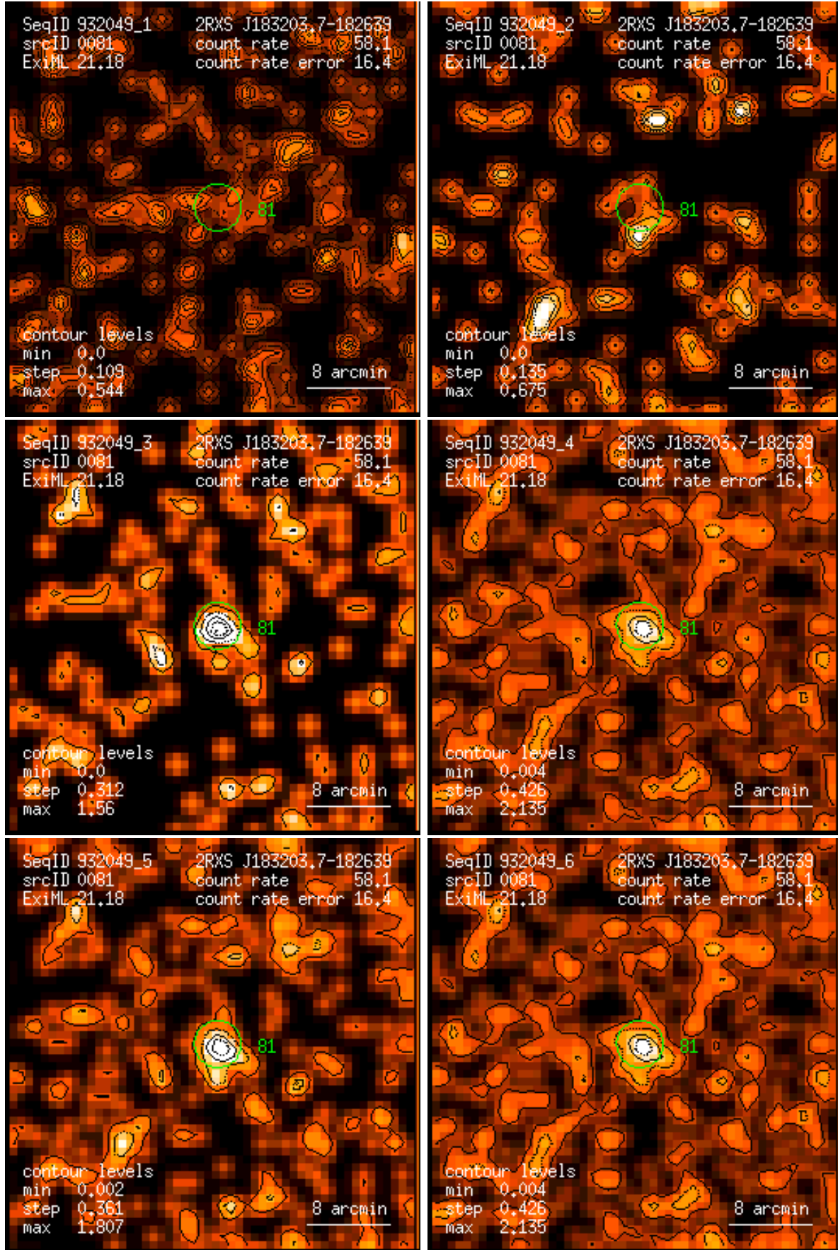
Figure 81: RASS 932049: detection 0081: band rate images, Gaussian filter: (1) PSPC channels 11 – 41, (2) 52 – 90, (3) 91 – 201, (4) 11 – 235, (5) 52 – 201, (6) 11 – 201. Broad band rates in counts/ks. Band rate contour levels in counts/ks/arcmin 2 .
