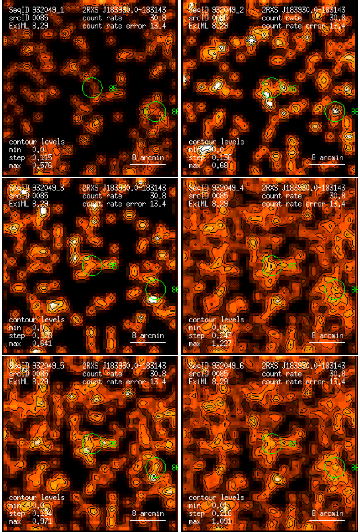
Figure 85: RASS 932049: detection 0085: band rate images, Gaussian filter: (1) PSPC channels 11 – 41, (2) 52 – 90, (3) 91 – 201, (4) 11 – 235, (5) 52 – 201, (6) 11 – 201. Broad band rates in counts/ks. Band rate contour levels in counts/ks/arcmin 2 .
