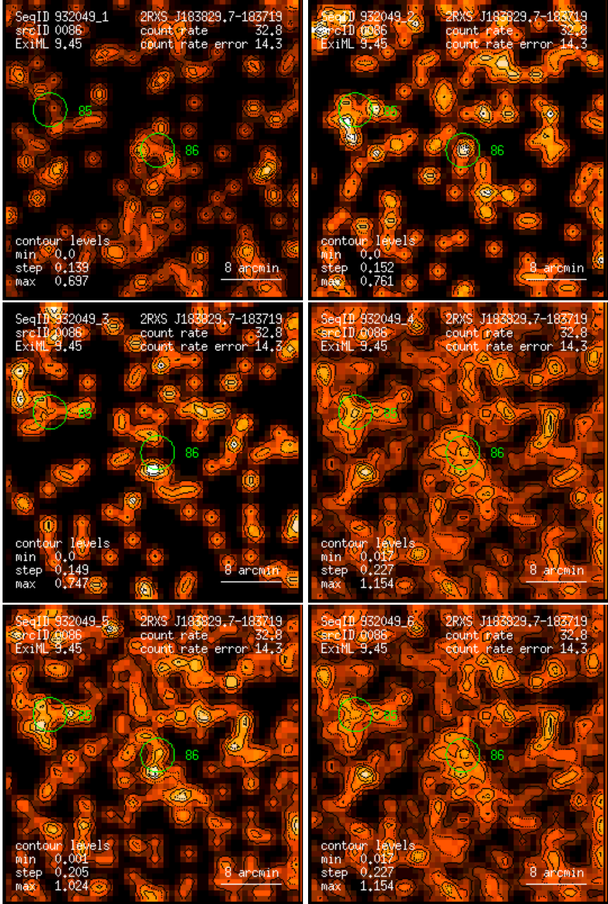
Figure 86: RASS 932049: detection 0086: band rate images, Gaussian filter: (1) PSPC channels 11 – 41, (2) 52 – 90, (3) 91 – 201, (4) 11 – 235, (5) 52 – 201, (6) 11 – 201. Broad band rates in counts/ks. Band rate contour levels in counts/ks/arcmin 2 .
