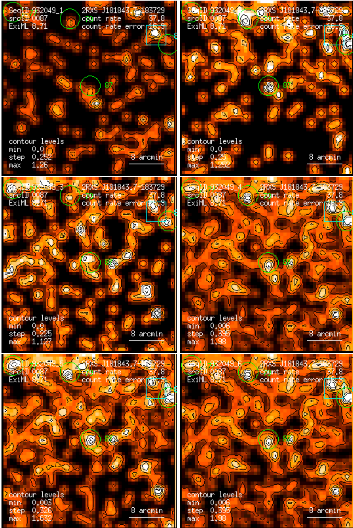
Figure 87: RASS 932049: detection 0087: band rate images, Gaussian filter: (1) PSPC channels 11 – 41, (2) 52 – 90, (3) 91 – 201, (4) 11 – 235, (5) 52 – 201, (6) 11 – 201. Broad band rates in counts/ks. Band rate contour levels in counts/ks/arcmin 2 .
