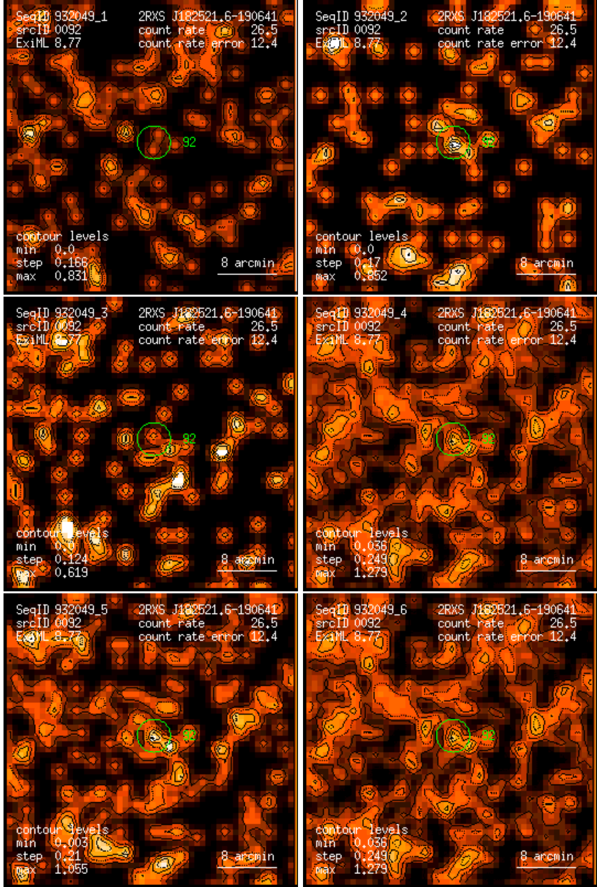
Figure 92: RASS 932049: detection 0092: band rate images, Gaussian filter: (1) PSPC channels 11 – 41, (2) 52 – 90, (3) 91 – 201, (4) 11 – 235, (5) 52 – 201, (6) 11 – 201. Broad band rates in counts/ks. Band rate contour levels in counts/ks/arcmin 2 .
