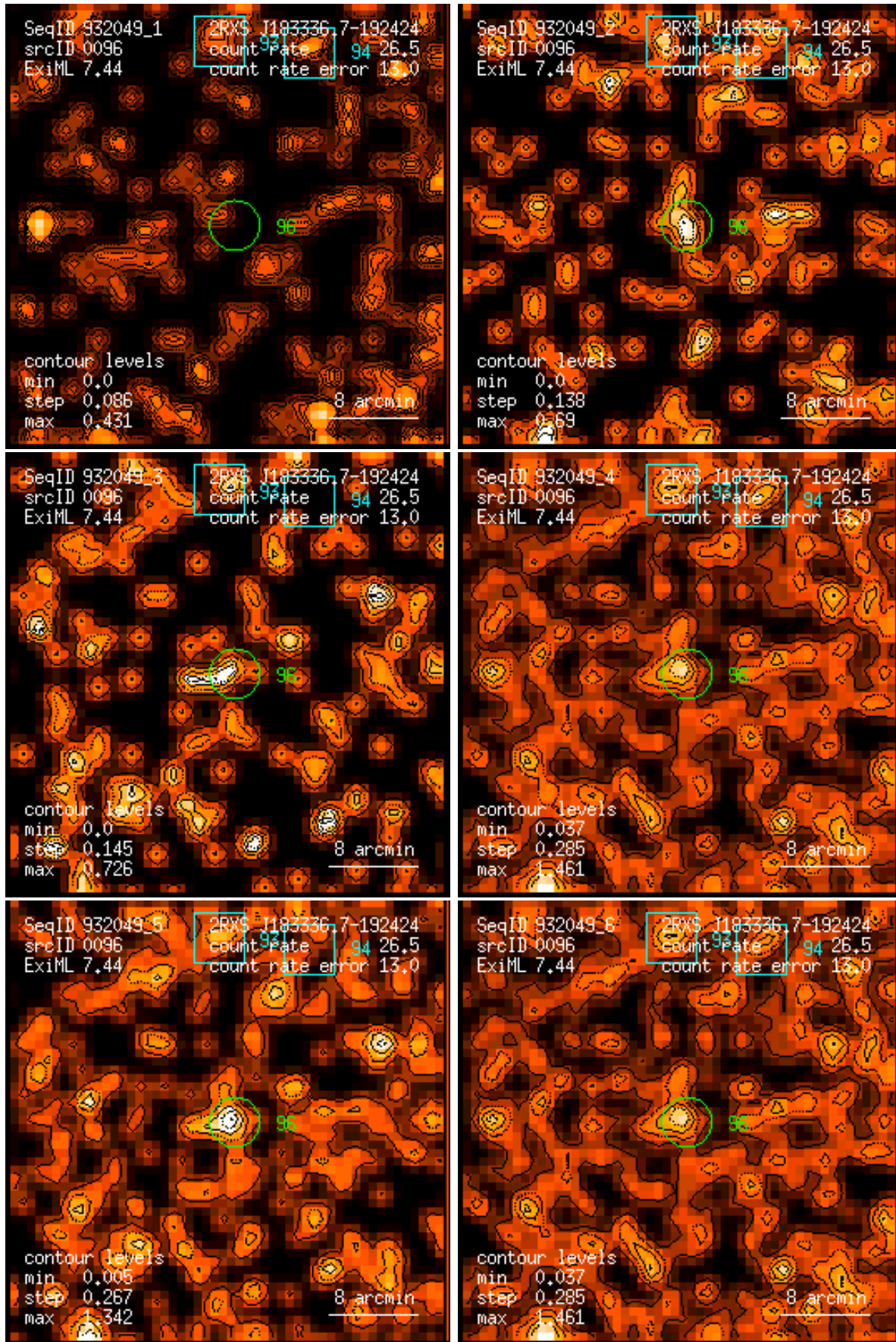
Figure 96: RASS 932049: detection 0096: band rate images, Gaussian filter: (1) PSPC channels 11 – 41, (2) 52 – 90, (3) 91 – 201, (4) 11 – 235, (5) 52 – 201, (6) 11 – 201. Broad band rates in counts/ks. Band rate contour levels in counts/ks/arcmin 2 .
