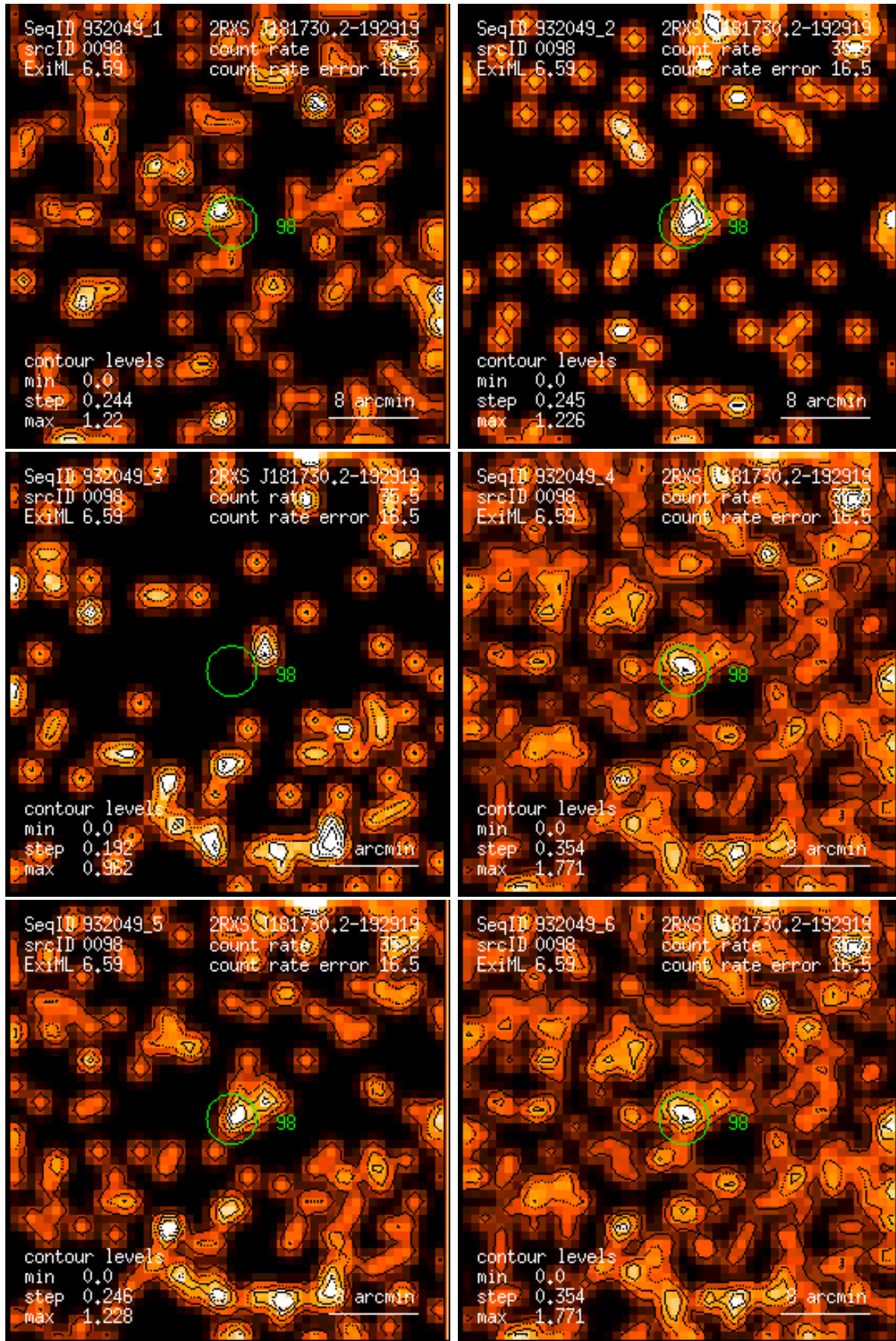
Figure 98: RASS 932049: detection 0098: band rate images, Gaussian filter: (1) PSPC channels 11 – 41, (2) 52 – 90, (3) 91 – 201, (4) 11 – 235, (5) 52 – 201, (6) 11 – 201. Broad band rates in counts/ks. Band rate contour levels in counts/ks/arcmin 2 .
