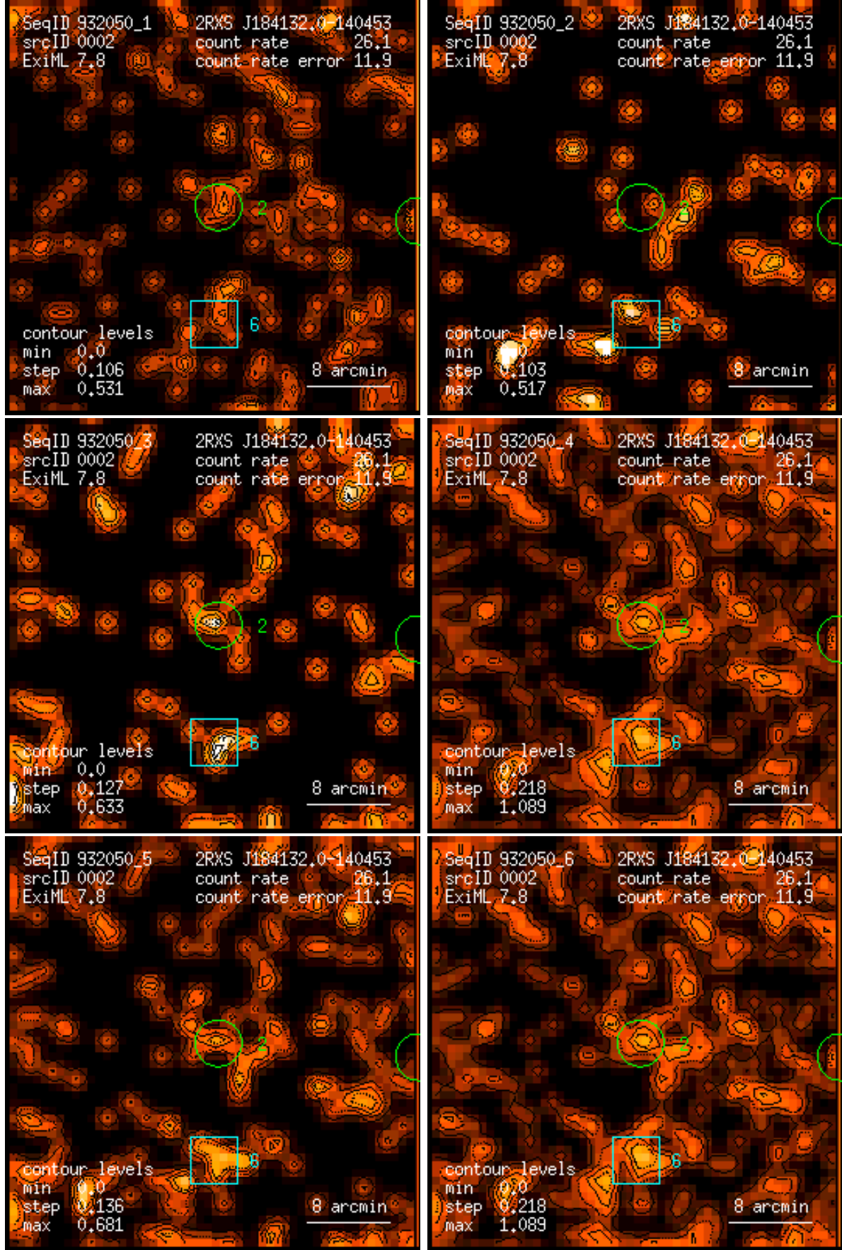
Figure 2: RASS 932050: detection 0002: band rate images, Gaussian filter: (1) PSPC channels 11 – 41, (2) 52 – 90, (3) 91 – 201, (4) 11 – 235, (5) 52 – 201, (6) 11 – 201. Broad band rates in counts/ks. Band rate contour levels in counts/ks/arcmin 2 .
