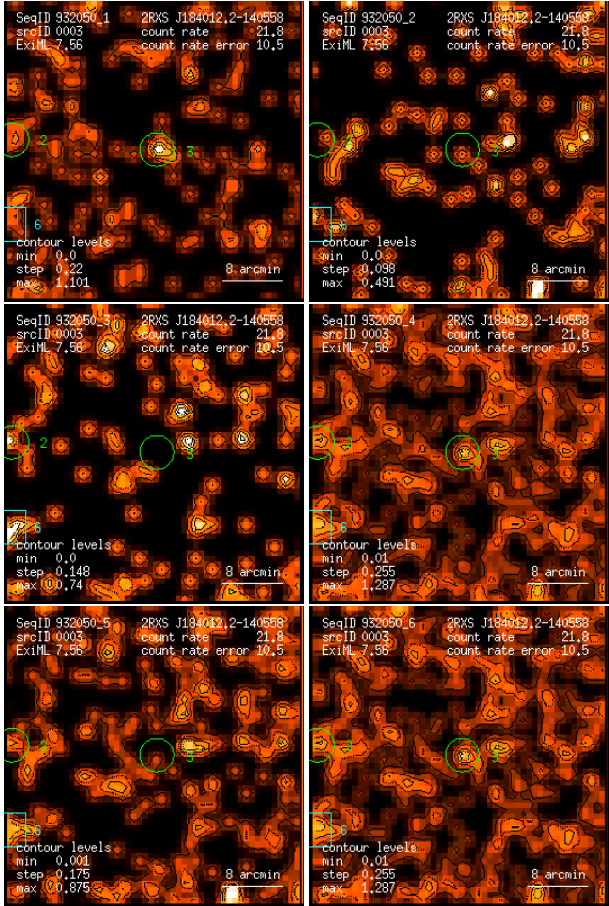
Figure 3: RASS 932050: detection 0003: band rate images, Gaussian filter: (1) PSPC channels 11 – 41, (2) 52 – 90, (3) 91 – 201, (4) 11 – 235, (5) 52 – 201, (6) 11 – 201. Broad band rates in counts/ks. Band rate contour levels in counts/ks/arcmin 2 .
