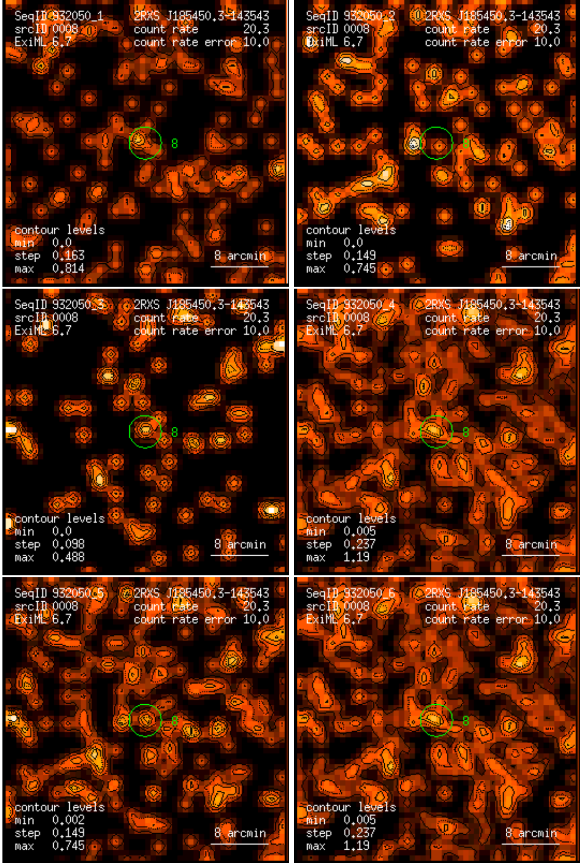
Figure 8: RASS 932050: detection 0008: band rate images, Gaussian filter: (1) PSPC channels 11 – 41, (2) 52 – 90, (3) 91 – 201, (4) 11 – 235, (5) 52 – 201, (6) 11 – 201. Broad band rates in counts/ks. Band rate contour levels in counts/ks/arcmin 2 .
