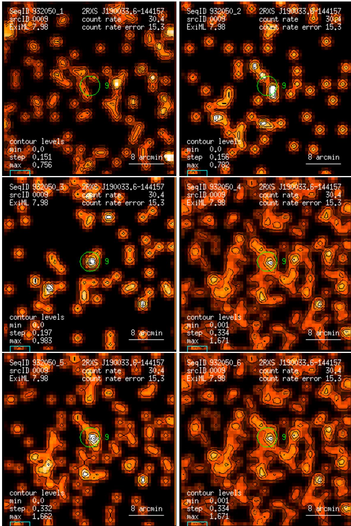
Figure 9: RASS 932050: detection 0009: band rate images, Gaussian filter: (1) PSPC channels 11 – 41, (2) 52 – 90, (3) 91 – 201, (4) 11 – 235, (5) 52 – 201, (6) 11 – 201. Broad band rates in counts/ks. Band rate contour levels in counts/ks/arcmin 2 .
