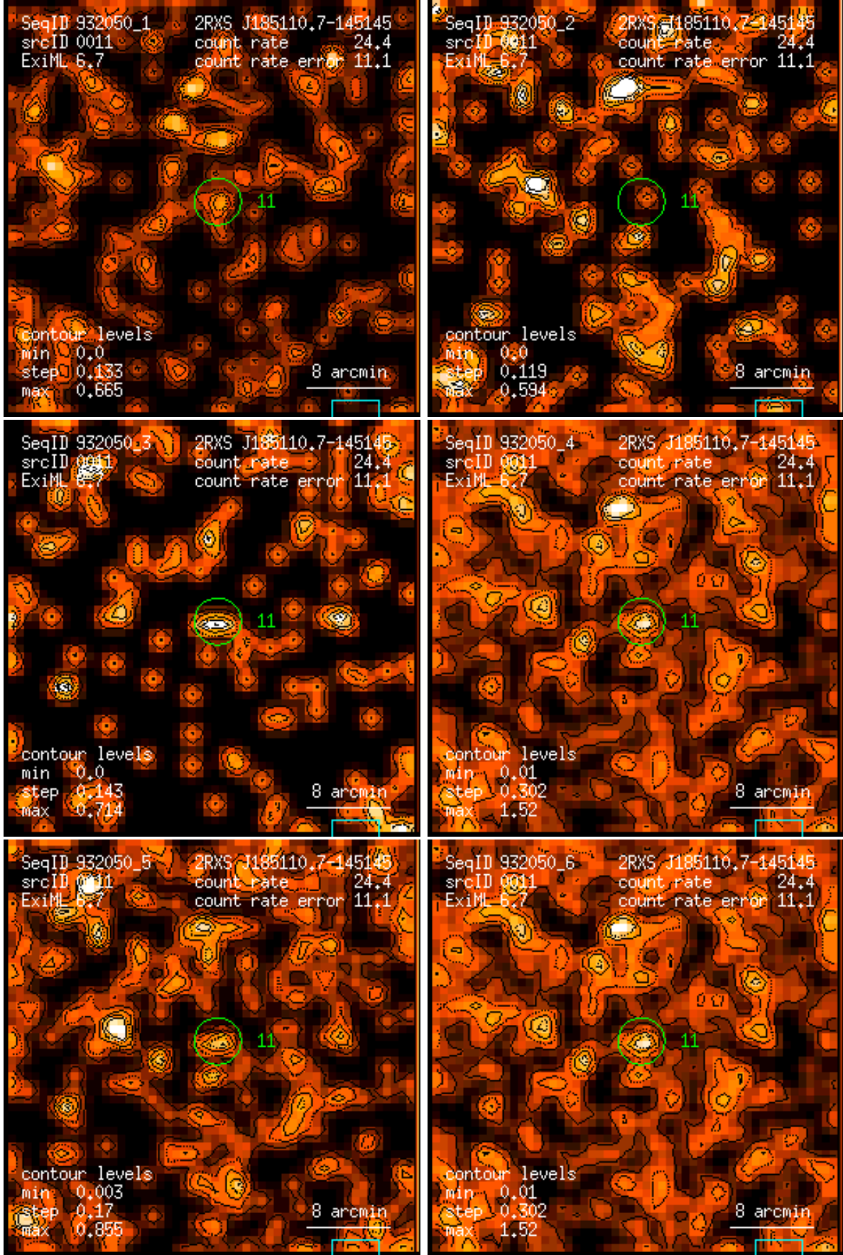
Figure 11: RASS 932050: detection 0011: band rate images, Gaussian filter: (1) PSPC channels 11 – 41, (2) 52 – 90, (3) 91 – 201, (4) 11 – 235, (5) 52 – 201, (6) 11 – 201. Broad band rates in counts/ks. Band rate contour levels in counts/ks/arcmin 2 .
