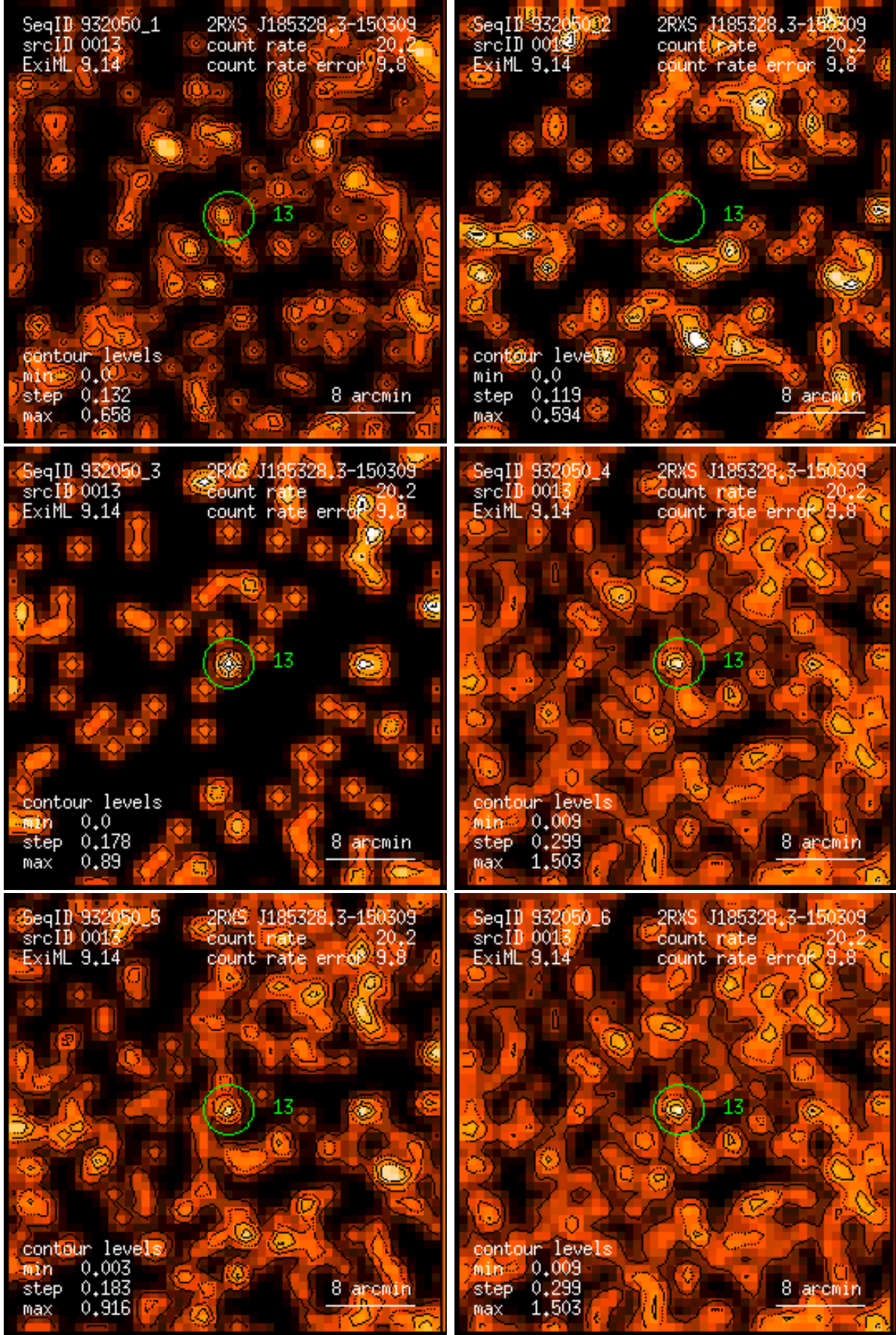
Figure 13: RASS 932050: detection 0013: band rate images, Gaussian filter: (1) PSPC channels 11 – 41, (2) 52 – 90, (3) 91 – 201, (4) 11 – 235, (5) 52 – 201, (6) 11 – 201. Broad band rates in counts/ks. Band rate contour levels in counts/ks/arcmin 2 .
