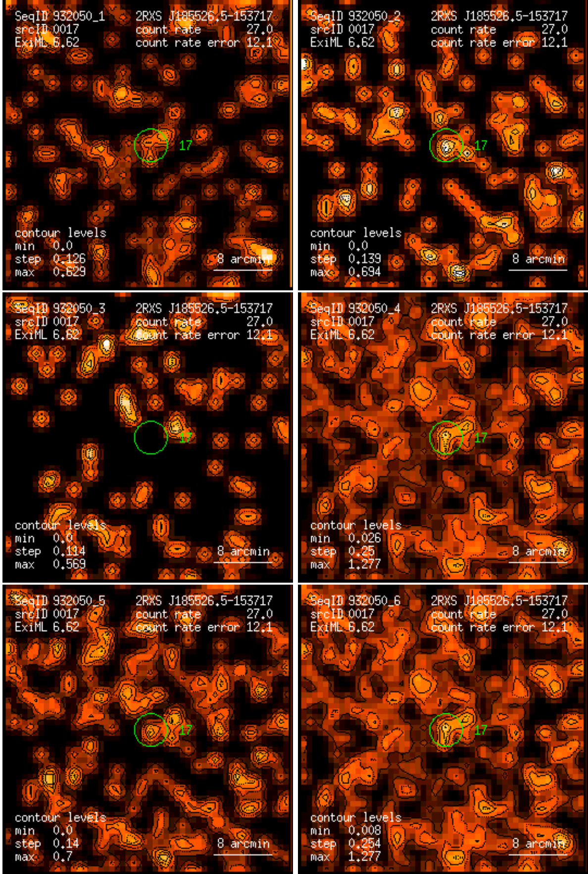
Figure 17: RASS 932050: detection 0017: band rate images, Gaussian filter: (1) PSPC channels 11 – 41, (2) 52 – 90, (3) 91 – 201, (4) 11 – 235, (5) 52 – 201, (6) 11 – 201. Broad band rates in counts/ks. Band rate contour levels in counts/ks/arcmin 2 .
