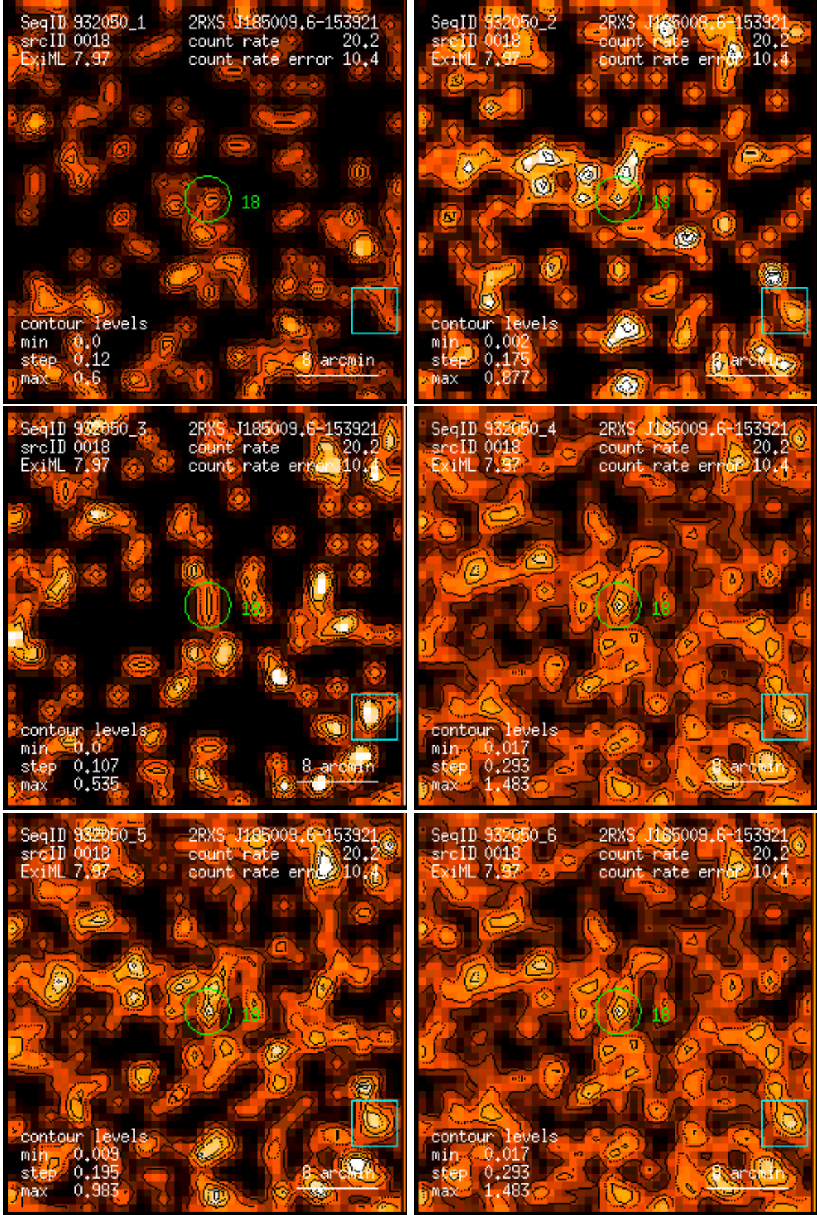
Figure 18: RASS 932050: detection 0018: band rate images, Gaussian filter: (1) PSPC channels 11 – 41, (2) 52 – 90, (3) 91 – 201, (4) 11 – 235, (5) 52 – 201, (6) 11 – 201. Broad band rates in counts/ks. Band rate contour levels in counts/ks/arcmin 2 .
