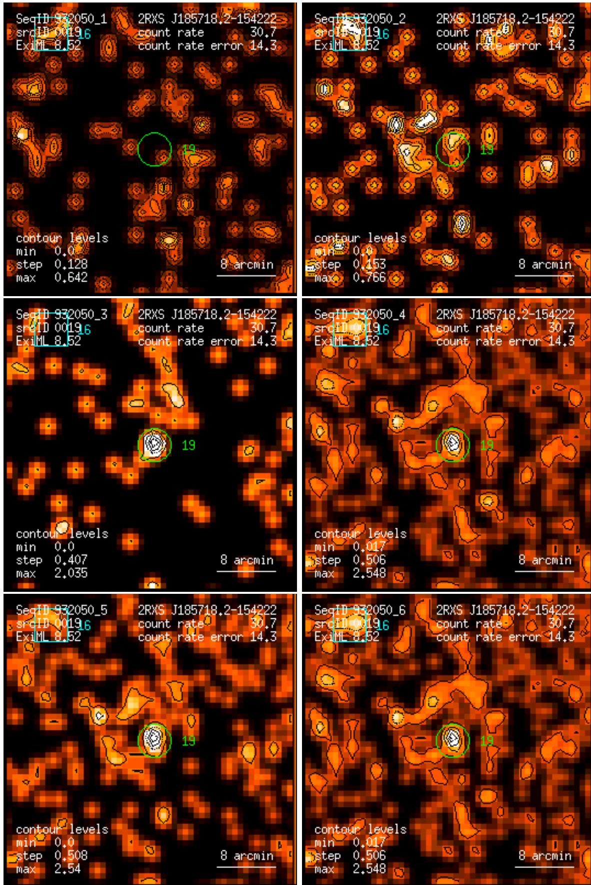
Figure 19: RASS 932050: detection 0019: band rate images, Gaussian filter: (1) PSPC channels 11 – 41, (2) 52 – 90, (3) 91 – 201, (4) 11 – 235, (5) 52 – 201, (6) 11 – 201. Broad band rates in counts/ks. Band rate contour levels in counts/ks/arcmin 2 .
