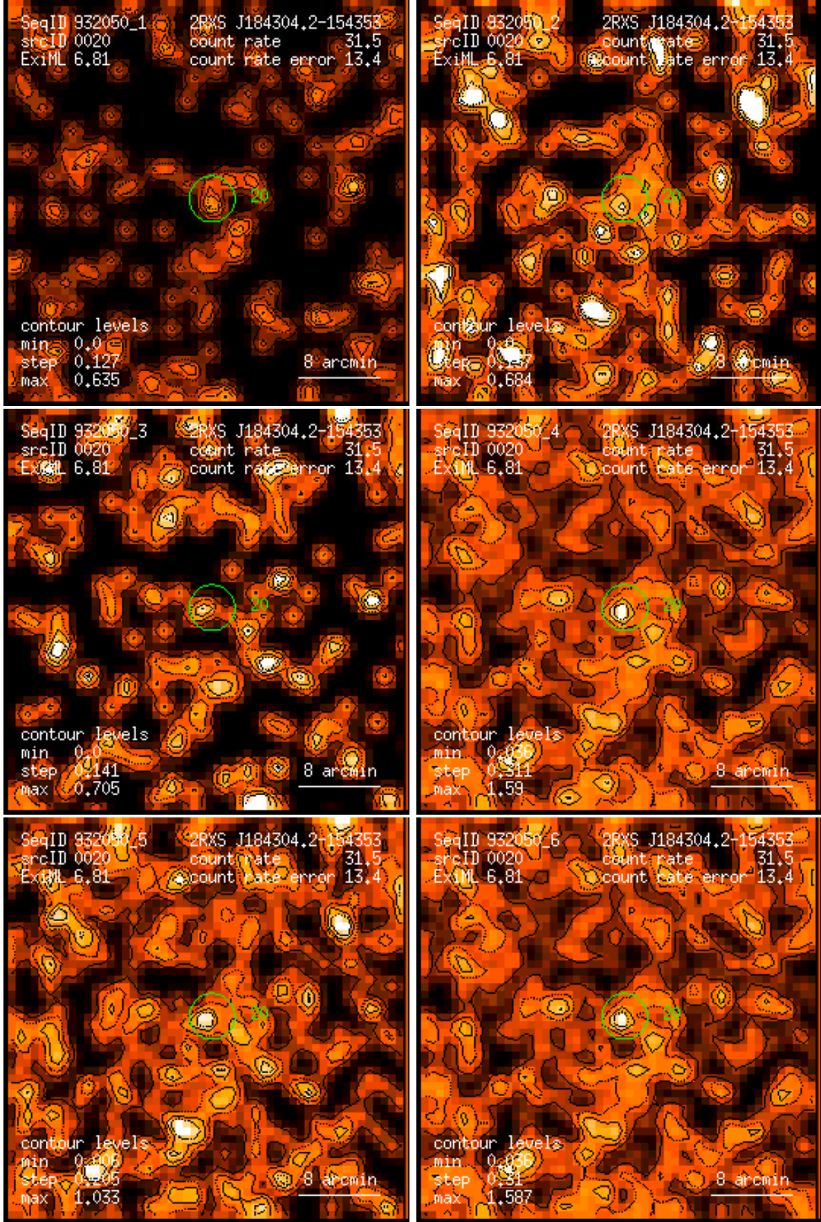
Figure 20: RASS 932050: detection 0020: band rate images, Gaussian filter: (1) PSPC channels 11 – 41, (2) 52 – 90, (3) 91 – 201, (4) 11 – 235, (5) 52 – 201, (6) 11 – 201. Broad band rates in counts/ks. Band rate contour levels in counts/ks/arcmin 2 .
