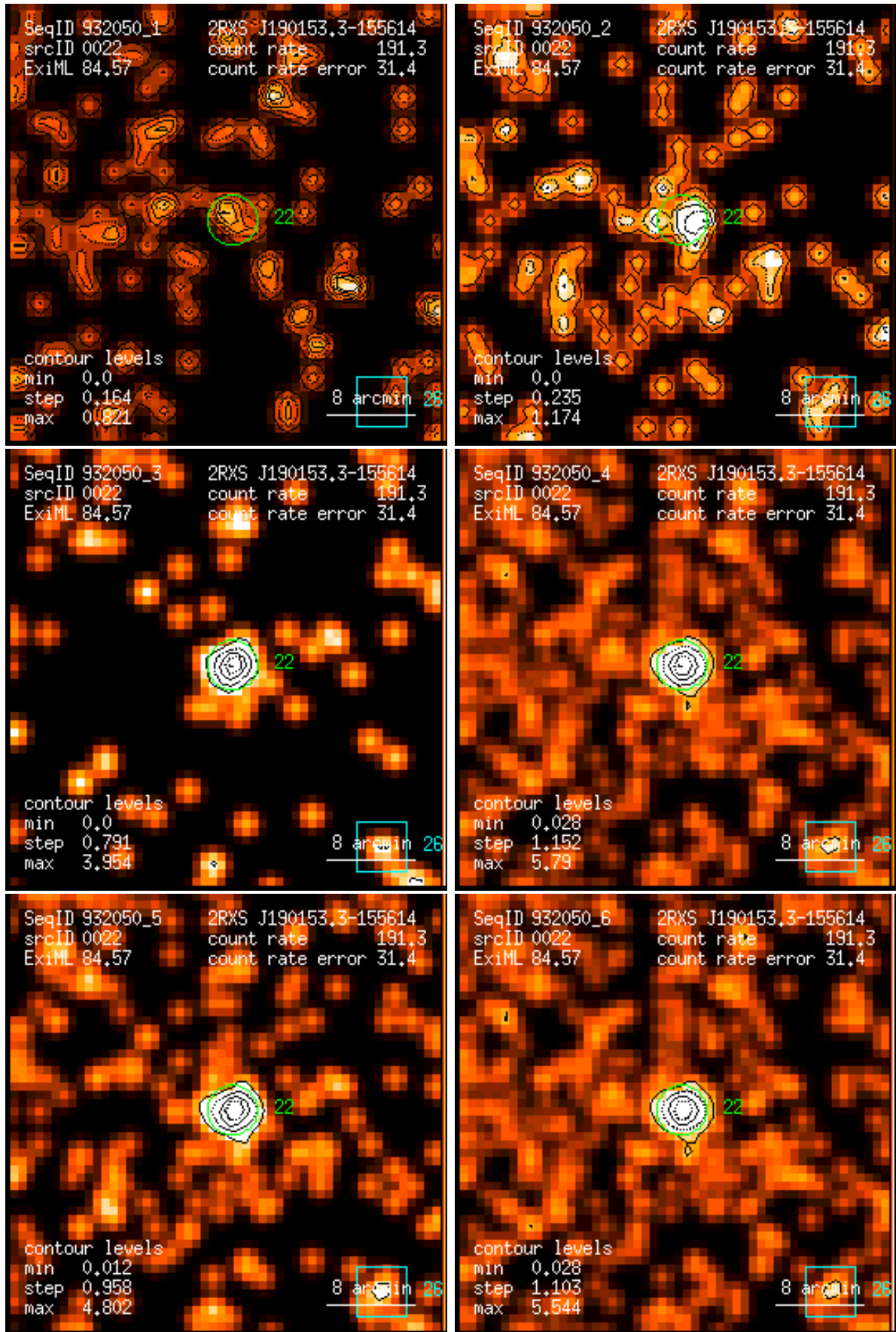
Figure 22: RASS 932050: detection 0022: band rate images, Gaussian filter: (1) PSPC channels 11 – 41, (2) 52 – 90, (3) 91 – 201, (4) 11 – 235, (5) 52 – 201, (6) 11 – 201. Broad band rates in counts/ks. Band rate contour levels in counts/ks/arcmin 2 .
