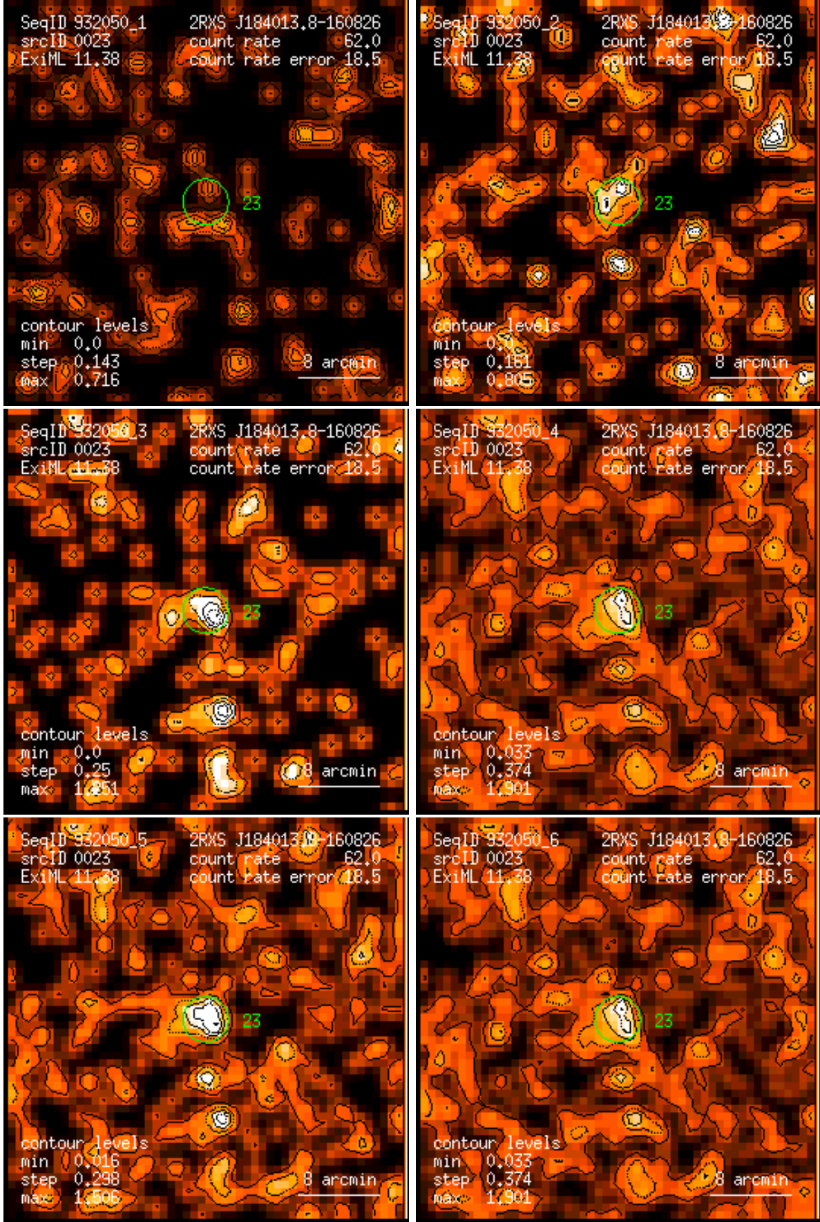
Figure 23: RASS 932050: detection 0023: band rate images, Gaussian filter: (1) PSPC channels 11 – 41, (2) 52 – 90, (3) 91 – 201, (4) 11 – 235, (5) 52 – 201, (6) 11 – 201. Broad band rates in counts/ks. Band rate contour levels in counts/ks/arcmin 2 .
