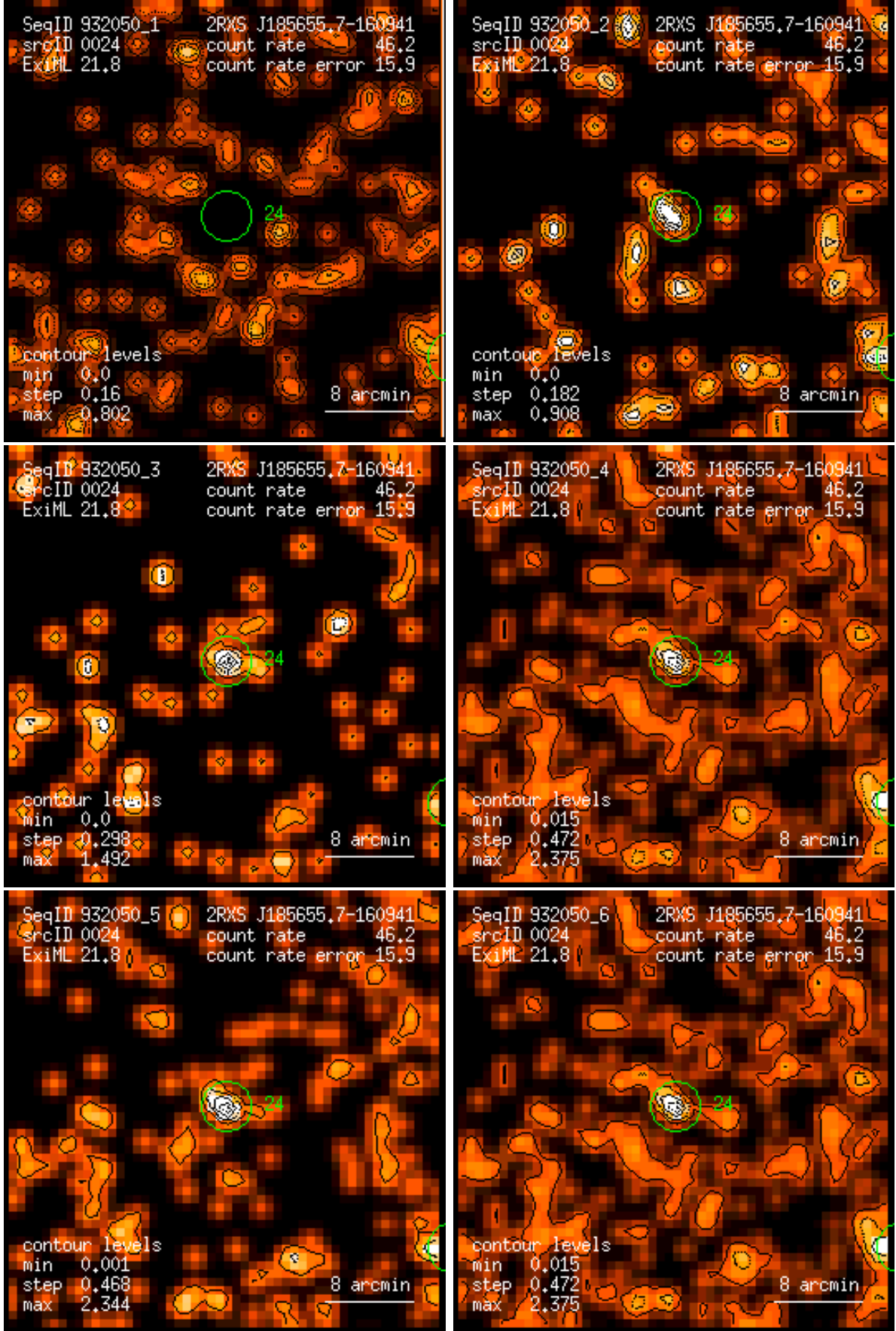
Figure 24: RASS 932050: detection 0024: band rate images, Gaussian filter: (1) PSPC channels 11 – 41, (2) 52 – 90, (3) 91 – 201, (4) 11 – 235, (5) 52 – 201, (6) 11 – 201. Broad band rates in counts/ks. Band rate contour levels in counts/ks/arcmin 2 .
