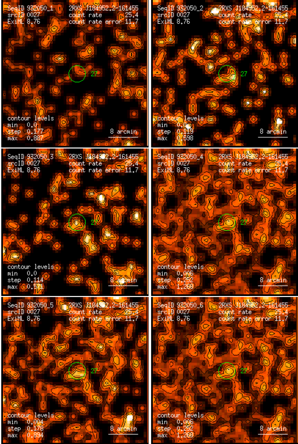
Figure 27: RASS 932050: detection 0027: band rate images, Gaussian filter: (1) PSPC channels 11 – 41, (2) 52 – 90, (3) 91 – 201, (4) 11 – 235, (5) 52 – 201, (6) 11 – 201. Broad band rates in counts/ks. Band rate contour levels in counts/ks/arcmin 2 .
