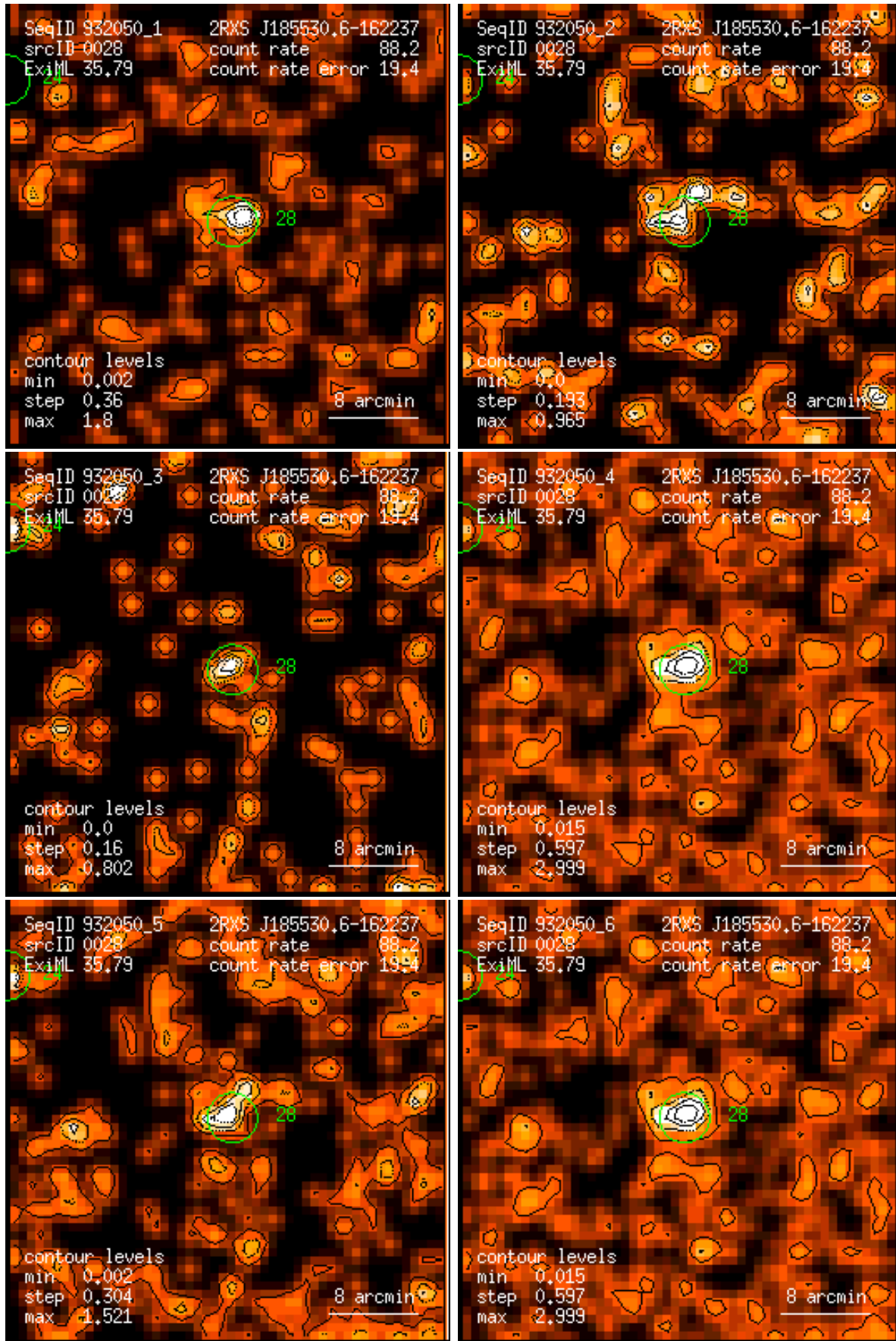
Figure 28: RASS 932050: detection 0028: band rate images, Gaussian filter: (1) PSPC channels 11 – 41, (2) 52 – 90, (3) 91 – 201, (4) 11 – 235, (5) 52 – 201, (6) 11 – 201. Broad band rates in counts/ks. Band rate contour levels in counts/ks/arcmin 2 .
