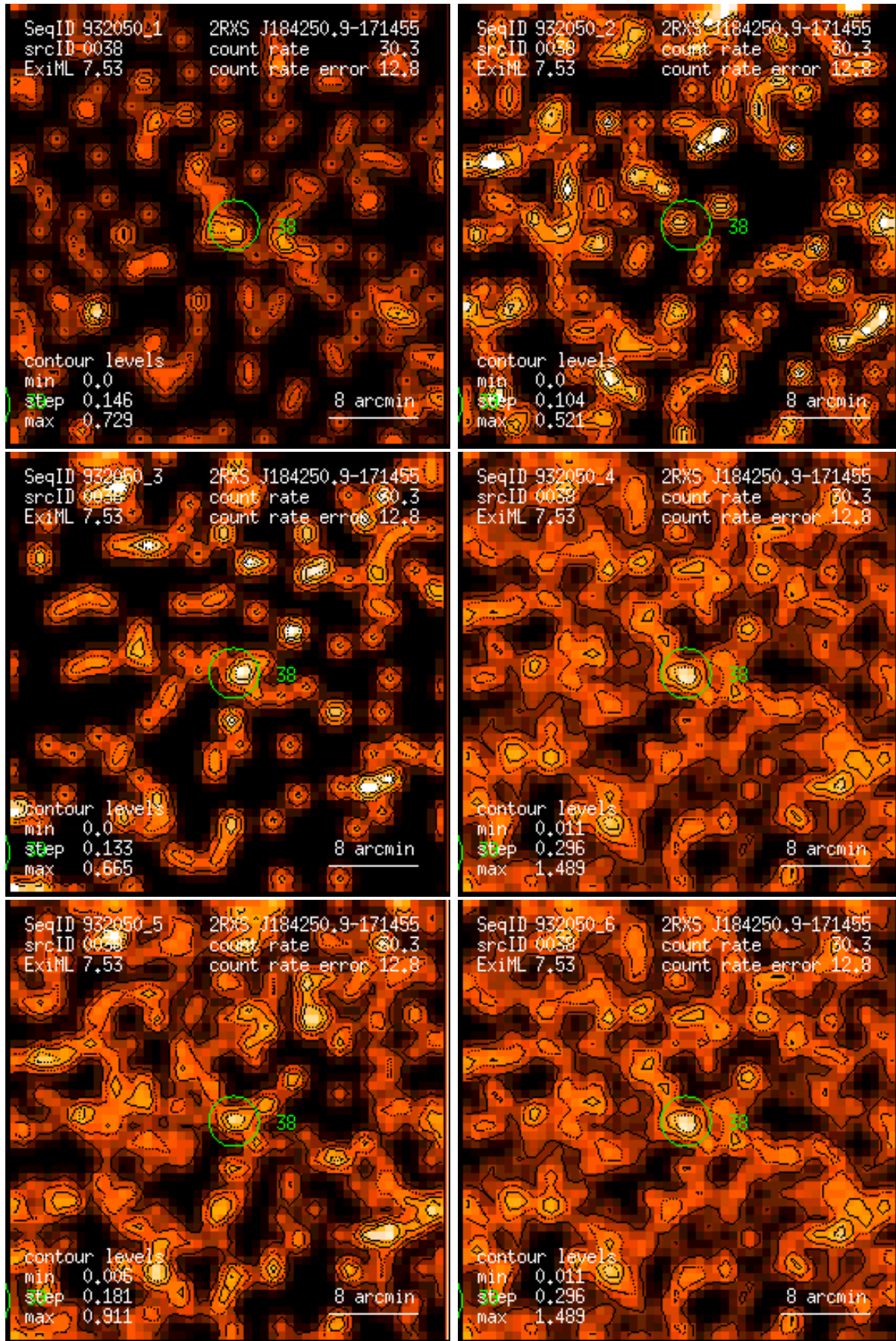
Figure 38: RASS 932050: detection 0038: band rate images, Gaussian filter: (1) PSPC channels 11 – 41, (2) 52 – 90, (3) 91 – 201, (4) 11 – 235, (5) 52 – 201, (6) 11 – 201. Broad band rates in counts/ks. Band rate contour levels in counts/ks/arcmin 2 .
