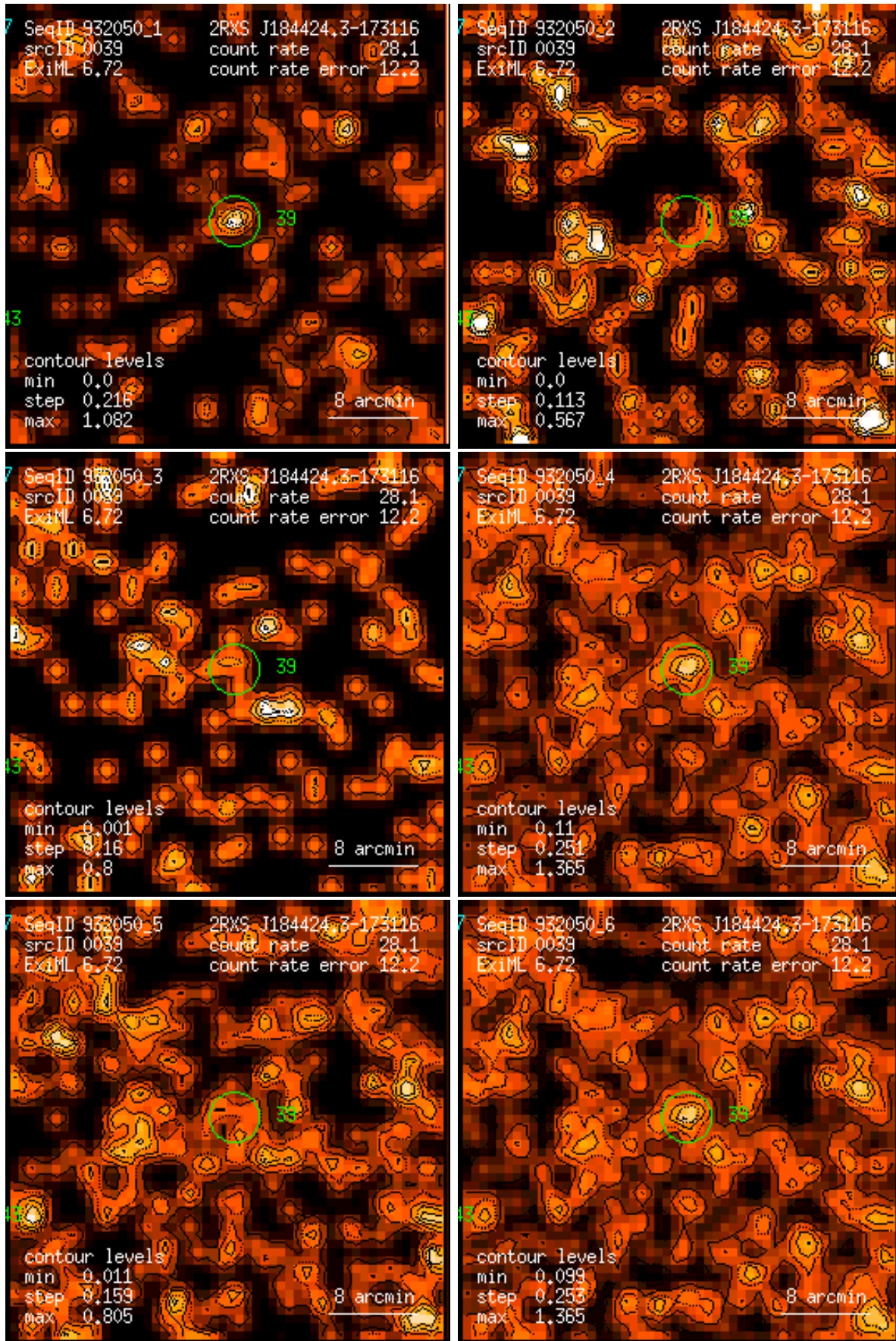
Figure 39: RASS 932050: detection 0039: band rate images, Gaussian filter: (1) PSPC channels 11 – 41, (2) 52 – 90, (3) 91 – 201, (4) 11 – 235, (5) 52 – 201, (6) 11 – 201. Broad band rates in counts/ks. Band rate contour levels in counts/ks/arcmin 2 .
