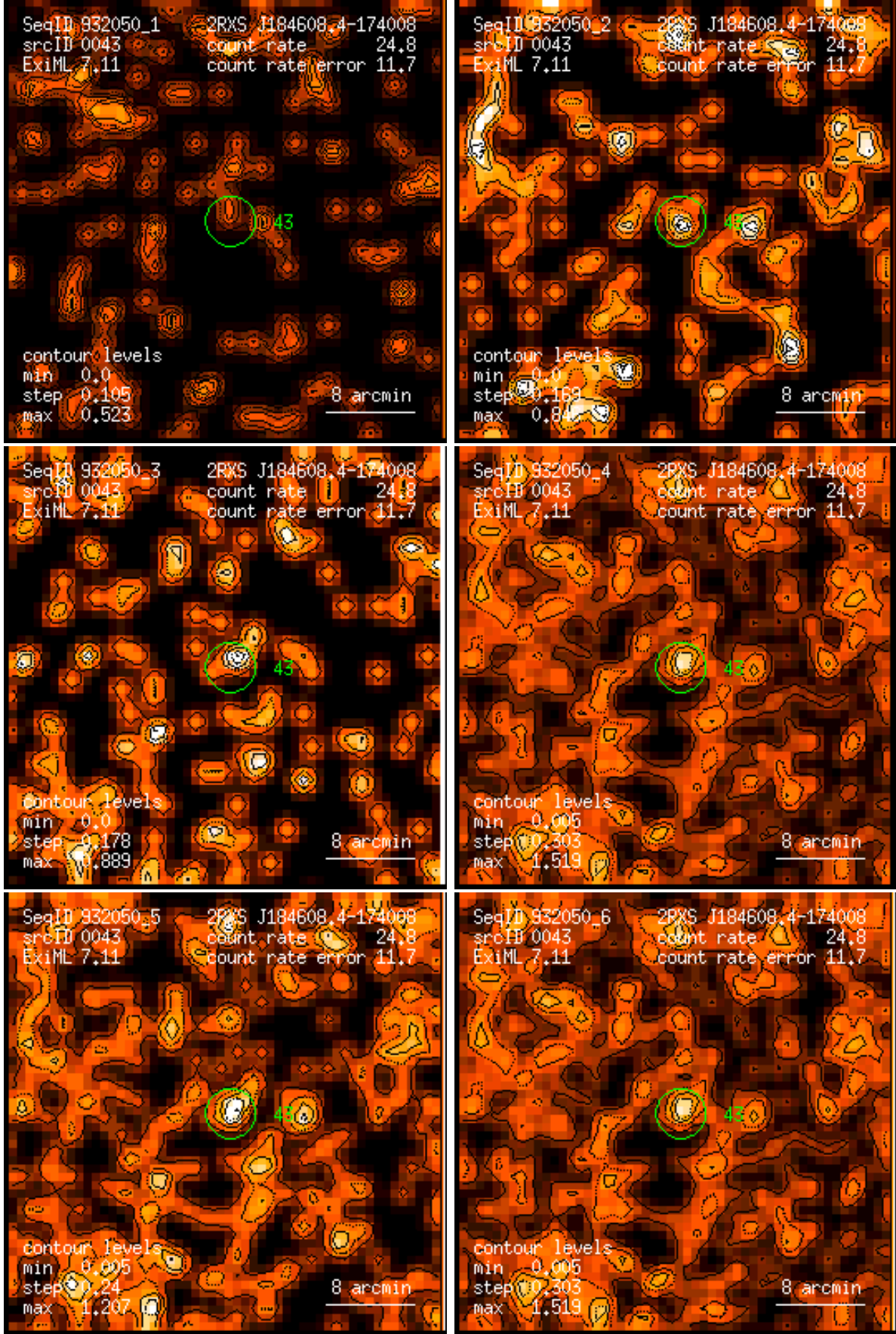
Figure 43: RASS 932050: detection 0043: band rate images, Gaussian filter: (1) PSPC channels 11 – 41, (2) 52 – 90, (3) 91 – 201, (4) 11 – 235, (5) 52 – 201, (6) 11 – 201. Broad band rates in counts/ks. Band rate contour levels in counts/ks/arcmin 2 .
