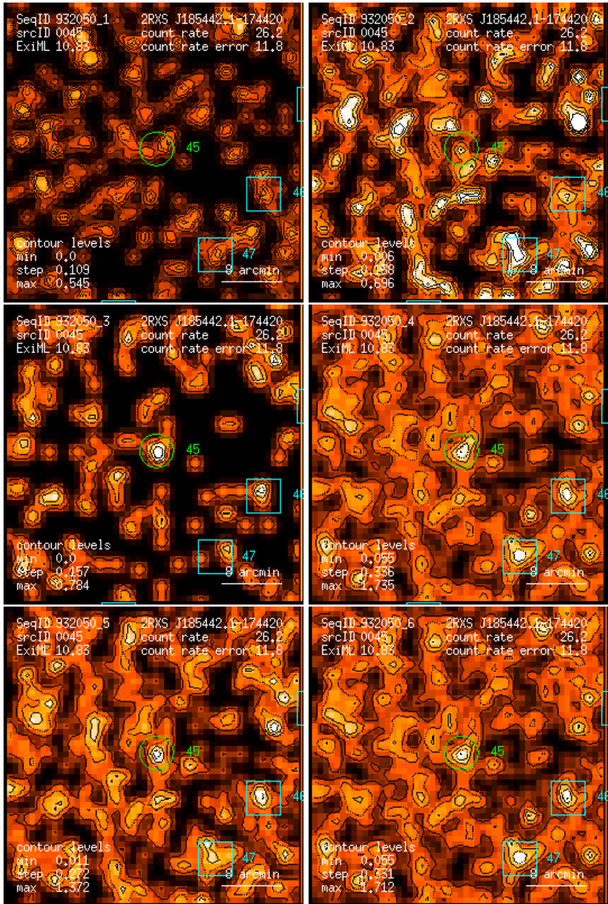
Figure 45: RASS 932050: detection 0045: band rate images, Gaussian filter: (1) PSPC channels 11 – 41, (2) 52 – 90, (3) 91 – 201, (4) 11 – 235, (5) 52 – 201, (6) 11 – 201. Broad band rates in counts/ks. Band rate contour levels in counts/ks/arcmin 2 .
