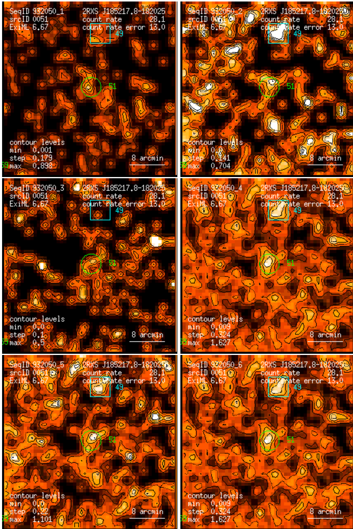
Figure 51: RASS 932050: detection 0051: band rate images, Gaussian filter: (1) PSPC channels 11 – 41, (2) 52 – 90, (3) 91 – 201, (4) 11 – 235, (5) 52 – 201, (6) 11 – 201. Broad band rates in counts/ks. Band rate contour levels in counts/ks/arcmin 2 .
