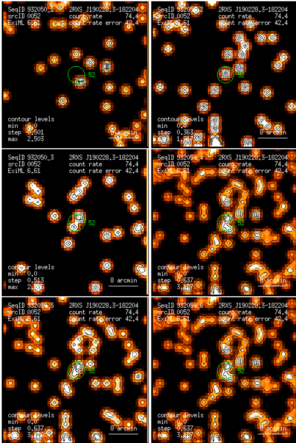
Figure 52: RASS 932050: detection 0052: band rate images, Gaussian filter: (1) PSPC channels 11 – 41, (2) 52 – 90, (3) 91 – 201, (4) 11 – 235, (5) 52 – 201, (6) 11 – 201. Broad band rates in counts/ks. Band rate contour levels in counts/ks/arcmin 2 .
