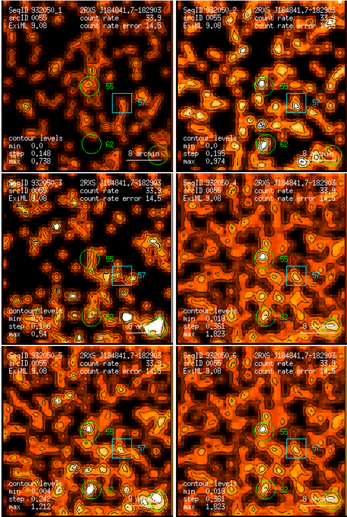
Figure 55: RASS 932050: detection 0055: band rate images, Gaussian filter: (1) PSPC channels 11 – 41, (2) 52 – 90, (3) 91 – 201, (4) 11 – 235, (5) 52 – 201, (6) 11 – 201. Broad band rates in counts/ks. Band rate contour levels in counts/ks/arcmin 2 .
