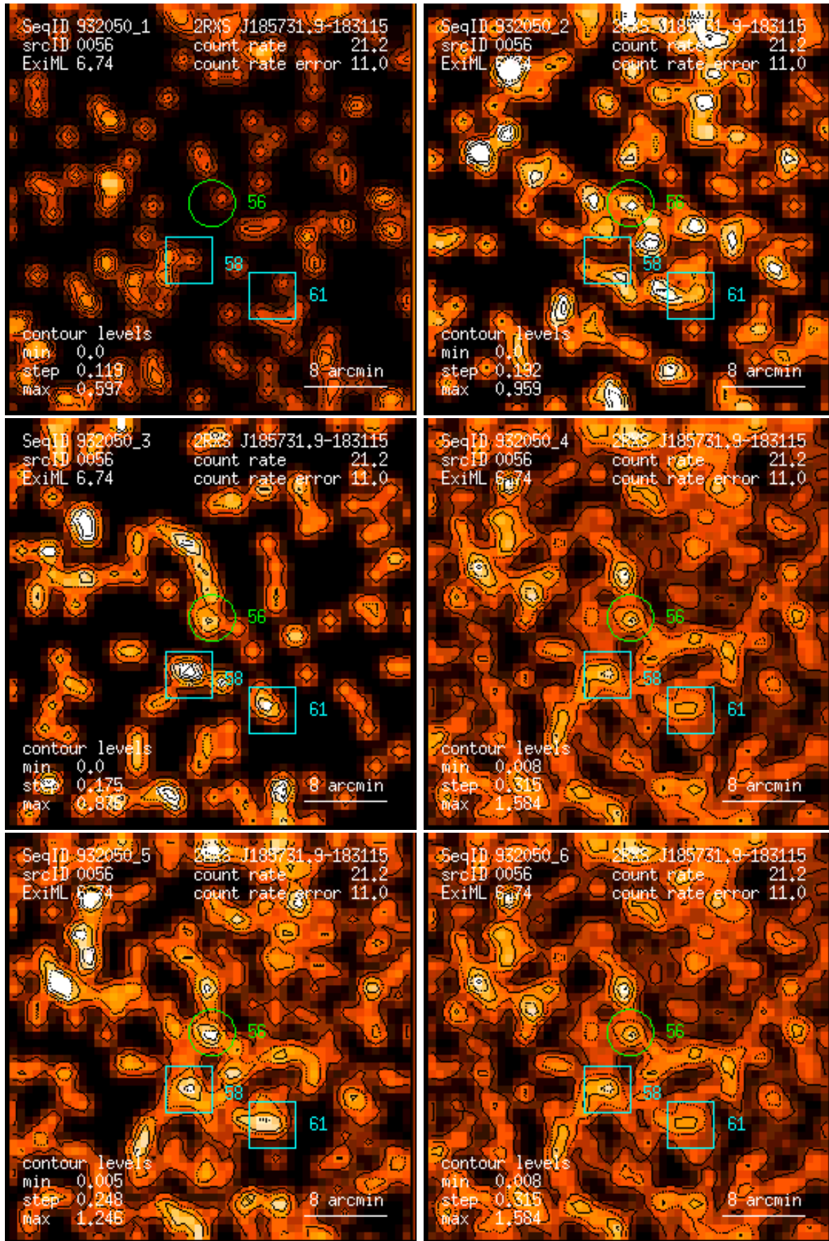
Figure 56: RASS 932050: detection 0056: band rate images, Gaussian filter: (1) PSPC channels 11 – 41, (2) 52 – 90, (3) 91 – 201, (4) 11 – 235, (5) 52 – 201, (6) 11 – 201. Broad band rates in counts/ks. Band rate contour levels in counts/ks/arcmin 2 .
